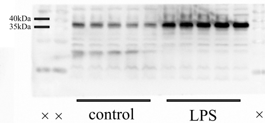
GAPDH 36 kDa
