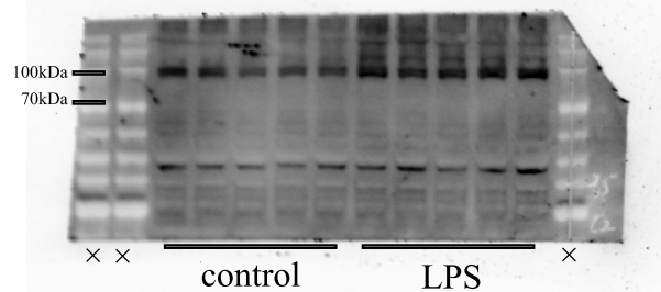
GAPDH 36 kDa
