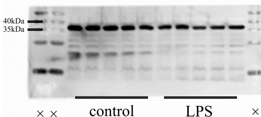
GAPDH 36 kDa
