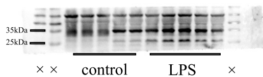
GAPDH 36 kDa
