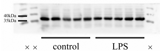
GAPDH 36 kDa
