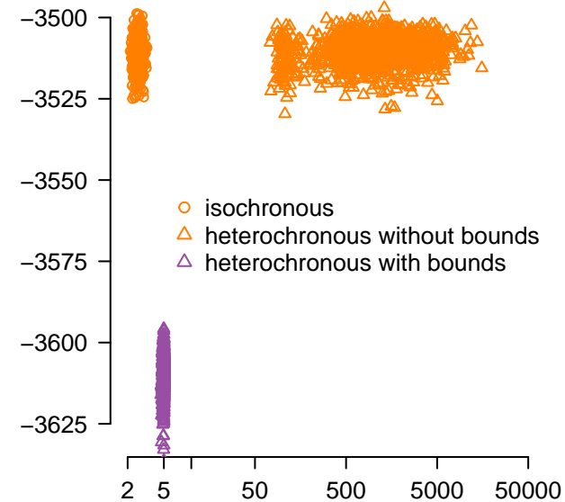
Isochronous, gamma prior
