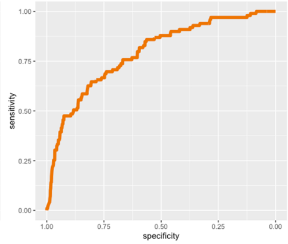
ROC Curve of predictors Month, Location, Weather, & Season (AUC = 0.79)
