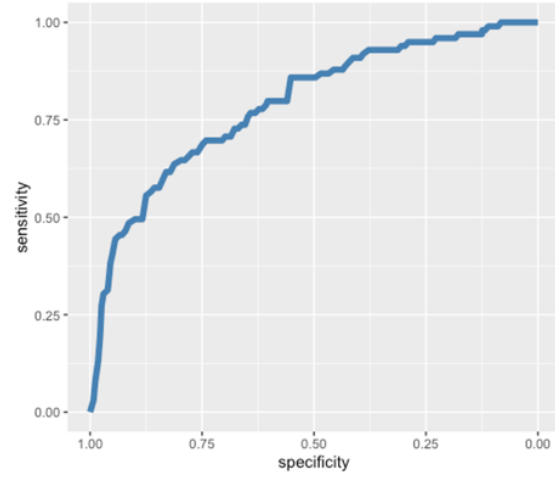
ROC Curve of predictors Month, Location & Season (AUC = 0.7904)
