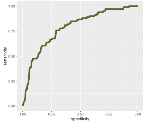
ROC Curve of predictors Month, Location & 30-day Rolling Averages of Minimum Temperature and Cum. Precipitation (AUC = 0.7859)
