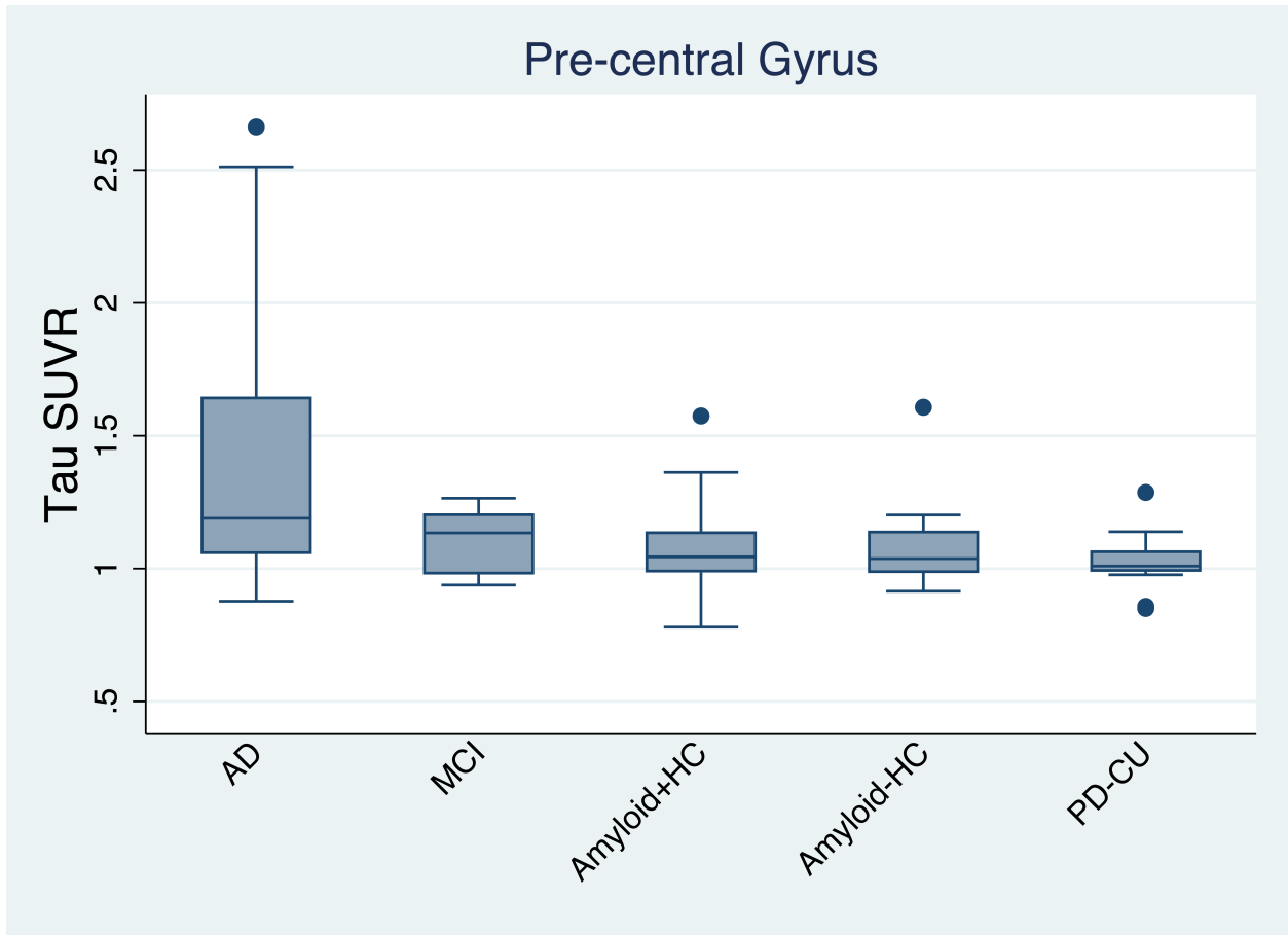
Figure S3: Tau uptake in the bilateral precentral gyri control reference region. There was a similar gradation of tau uptake ( p=0.003 ), but if the AD category was excluded, no significant difference existed ( p=0.172 ).
