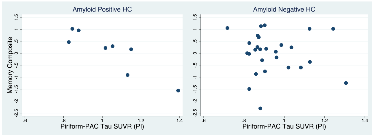
Figure S5: SAMS behavioral results. Left: The memory composite of Amyloid+HC showed a significant negative monotonic relationship relative to piriform-PAC tau uptake ( p=0.037 ). Right: Amyloid-HC showed no significant such relationship ( p>0.05 ).
