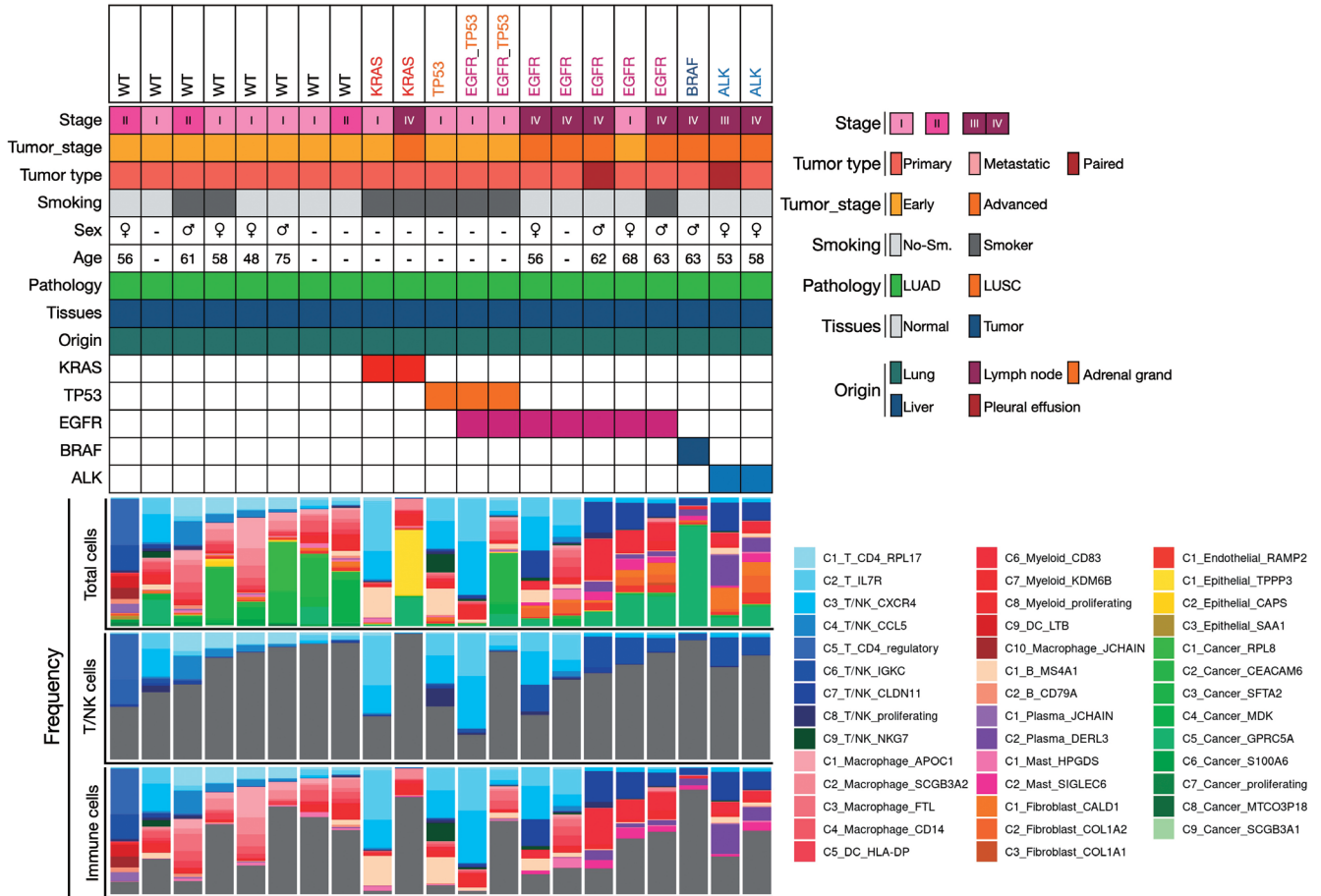
Supplementary Fig. 2. Stacked bar plots showing the clinical information of the 21 patients with primary tumor data and the proportion of the 41 clusters assigned a cell type for each patient. The three stacked bar plots represent the total cell types, T/NK cell types, and immune cell types, respectively.
