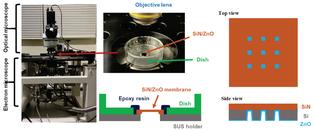
Figure S1 The photograph of the EXA-CL microscope and the pipeline of protocol of imaging of the micro/nanocrystals of proteins.
