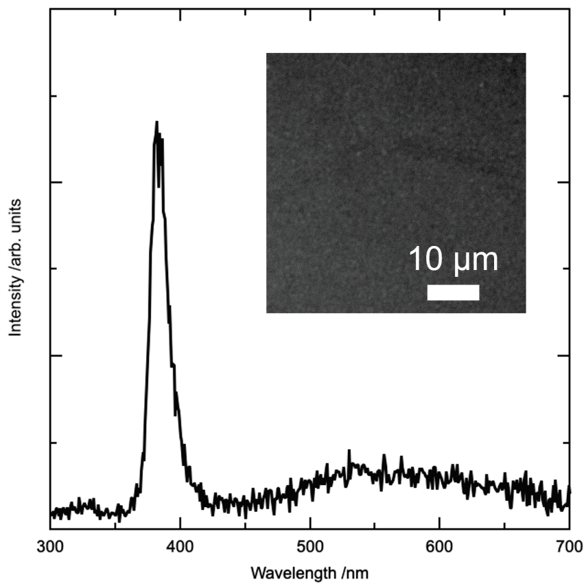
Figure S2 A typical cathodoluminescence spectra of ZnO. The inset shows the SEM image of the ZnO thin film.
