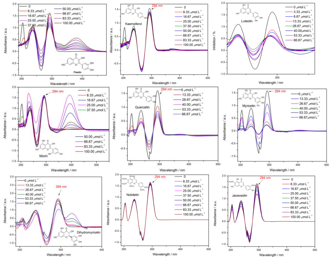
Fig S1 UV spectrums of bioflavonoids inhibiting XOD in vitro
