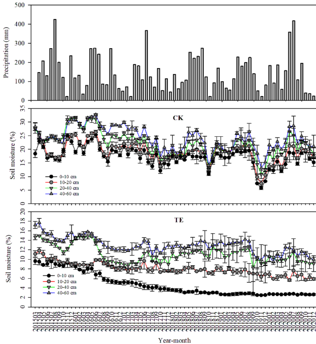
Figure 1S Precipitation and soil water moisture (0–60 cm) in drought-stressed plots (TE) and ambient controls (CK) across the drought-treatment experiment period in moso bamboo stands.
