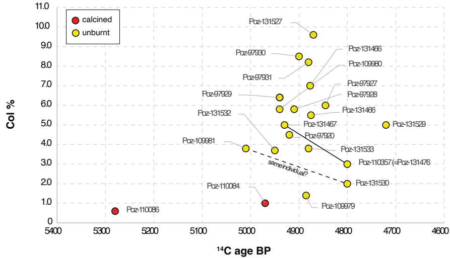
Figure 18: Collagen yield vs. 14 C result of human and faunal samples from the Kosenivka house 6 measured at the Radiocarbon Laboratory, Poznan (see S1 Tables).
