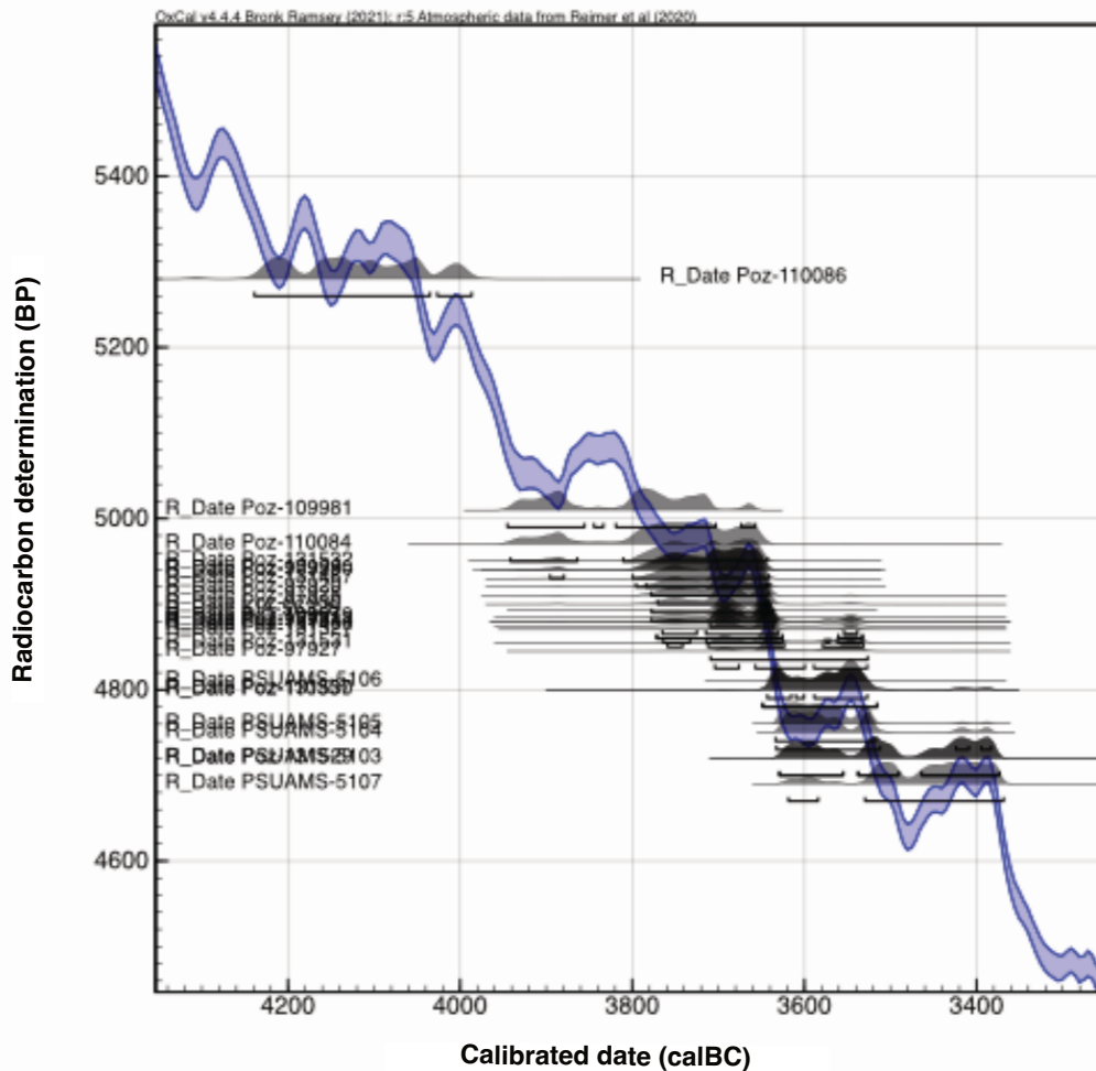
Figure 19: Calibration curve of all radiocarbon dates obtained for Kosenivka (n=26) using OxCal v. 4.4.
