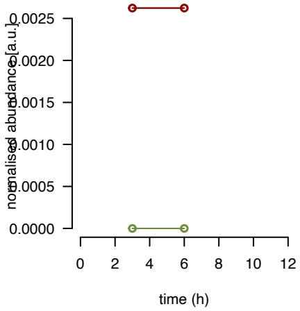
uL16m fraction 9
