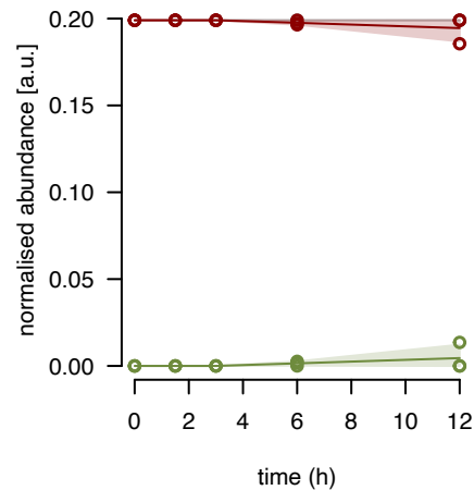
mL63 fraction 12
