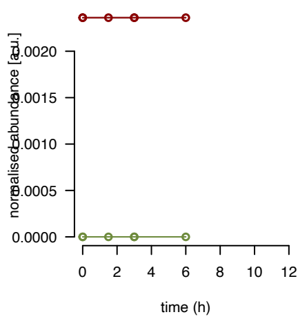
uL14m fraction 6
