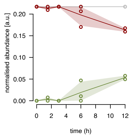
bL32m fraction 15
