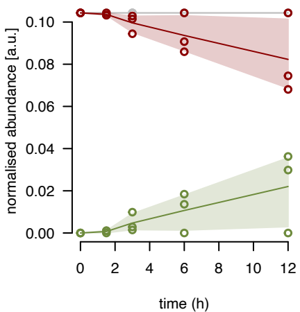
mL66 fraction 13
