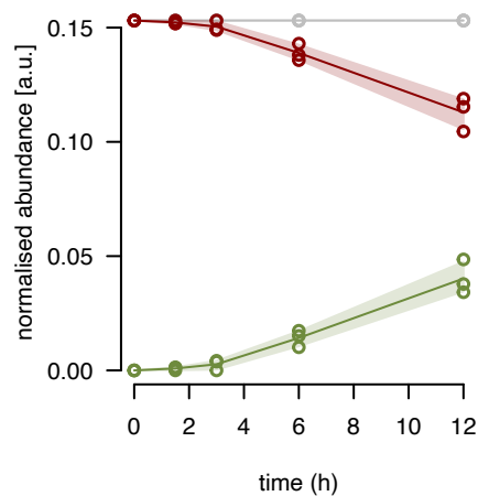
mL66 fraction 15
