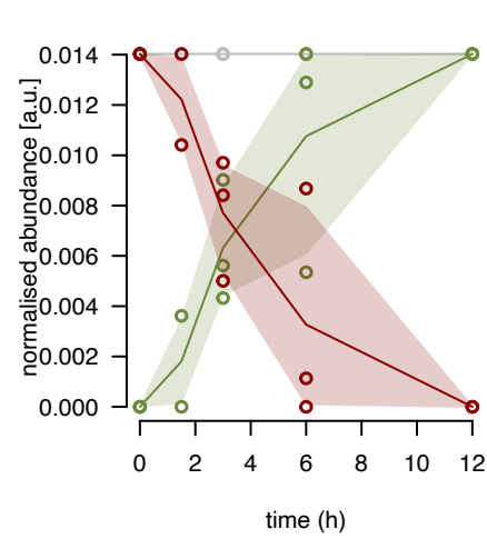
mL39 fraction 4
