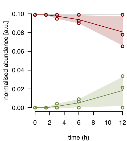
bL17m fraction 14
