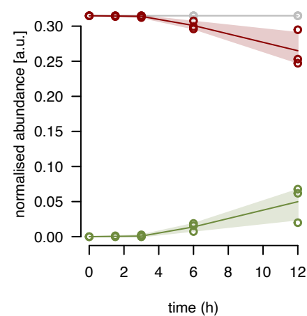
bL21m fraction 12
