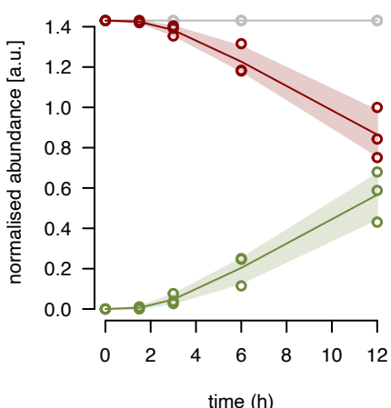
mL43 fraction 9
