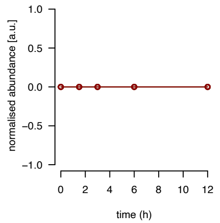
bL35m fraction 4
