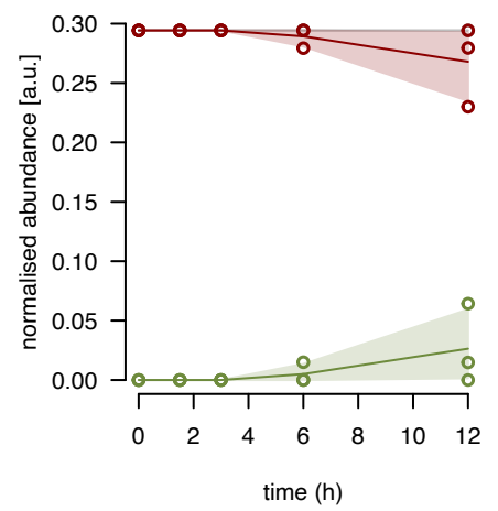
uL14m fraction 12
