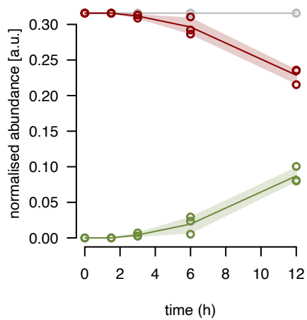
uL29m fraction 10
