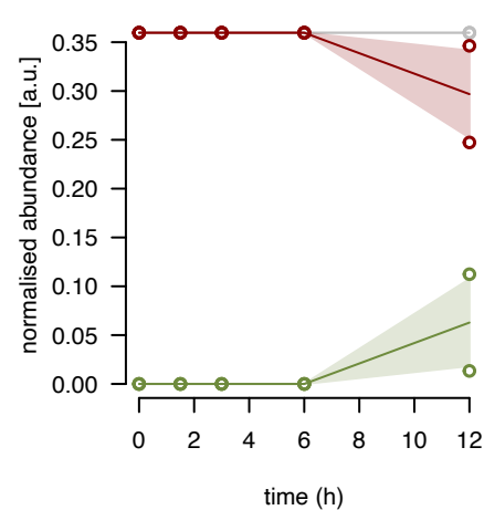
mL53 fraction 12
