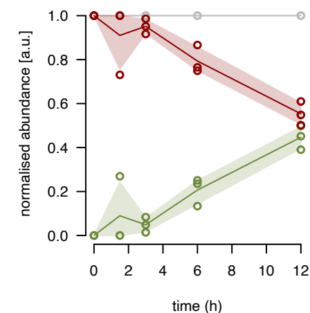
mL49 fraction 8
