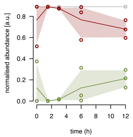
uL22m fraction 16
