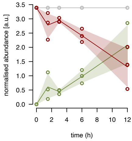
uL10m fraction 2
