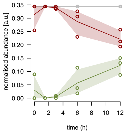
uL22m fraction 10
