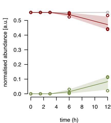
mL50 fraction 11
