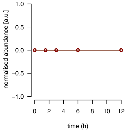
uL16m fraction 6
