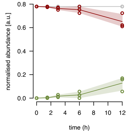
bL21m fraction 16
