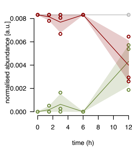
mL39 fraction 7
