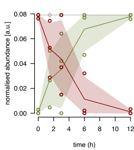
mL39 fraction 3
