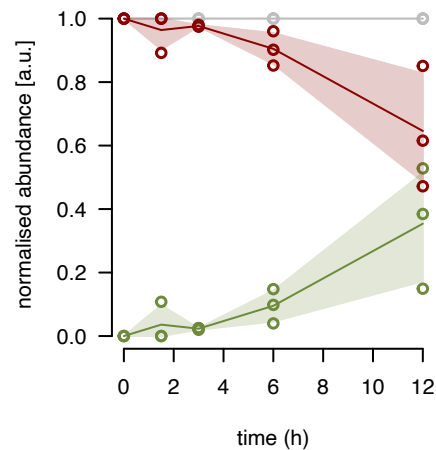
mL63 fraction 8
