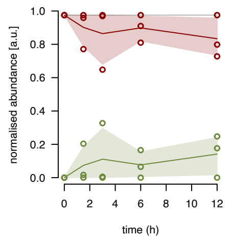
uL30m fraction 16
