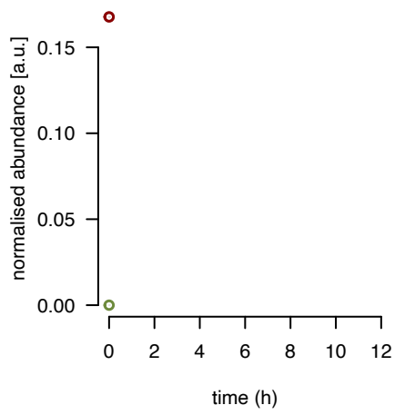
bL33m fraction 2
