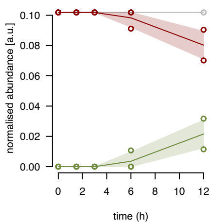
mL62 fraction 15
