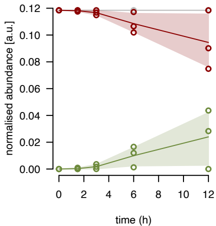
uL24m fraction 14
