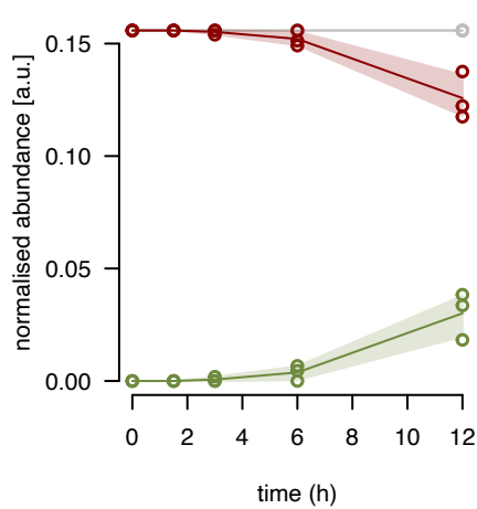
uL14m fraction 14
