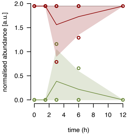
bL35m fraction 13
