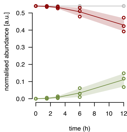
uL24m fraction 11
