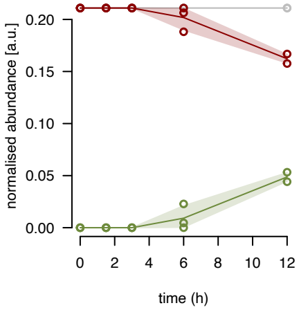
uL16m fraction 13
