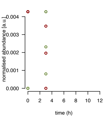
mL39 fraction 5
