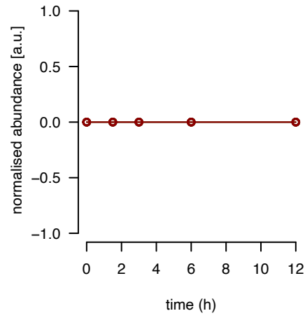
bL33m fraction 11
