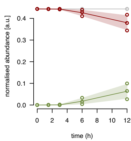
uL1m fraction 11
