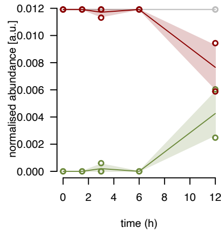
uL18m fraction 7
