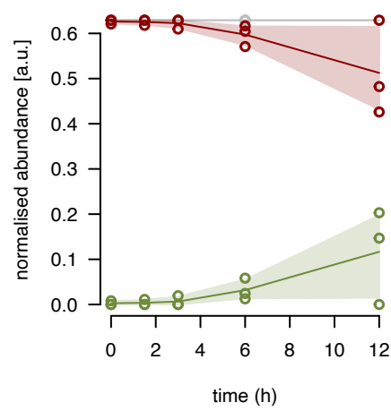
bL32m fraction 11
