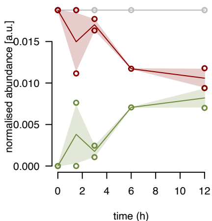
mL43 fraction 6
