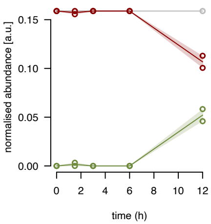
bL32m fraction 13
