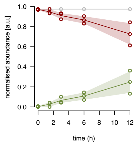
uL3m fraction 16
