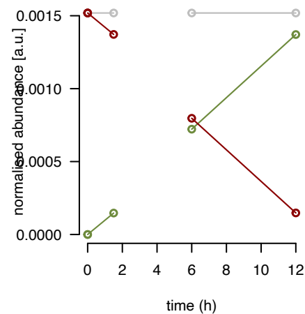
mL66 fraction 4
