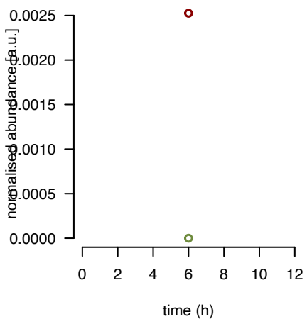
mL63 fraction 5
