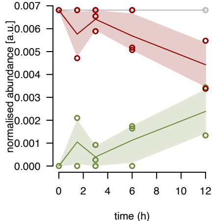
mL43 fraction 7
