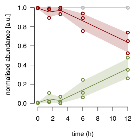
uL1m fraction 8
