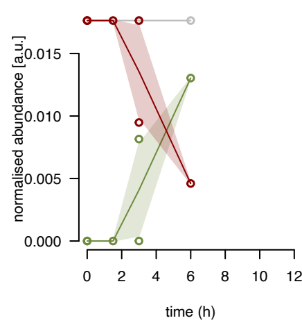
uL14m fraction 3
