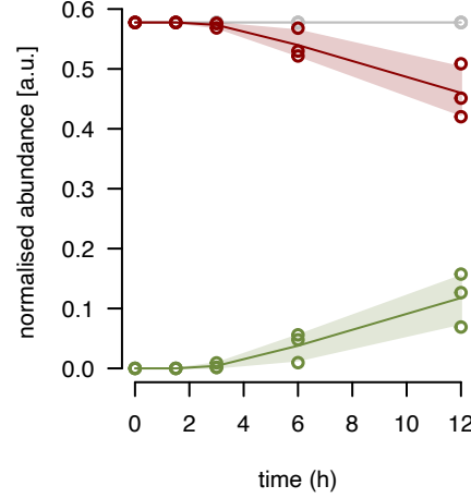
uL4m fraction 11
