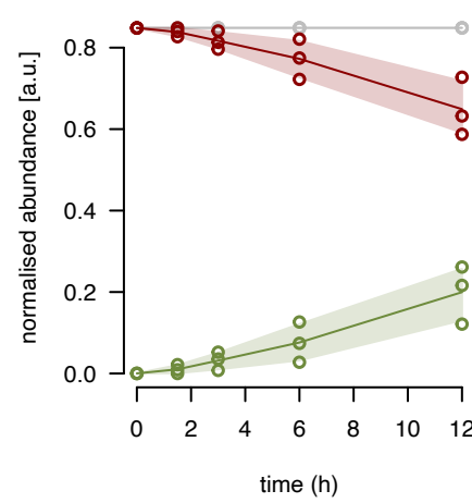
bL19m fraction 16
