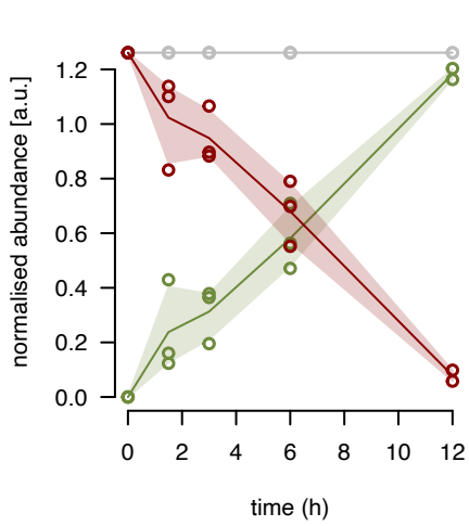
mL40 fraction 2
