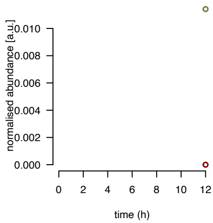
bL35m fraction 2
