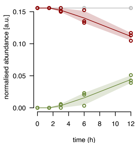
uL13m fraction 14
