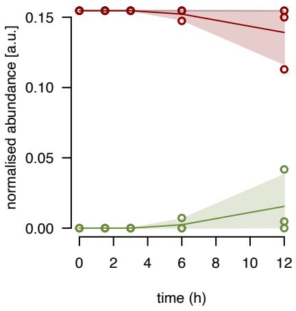
mL44 fraction 13
