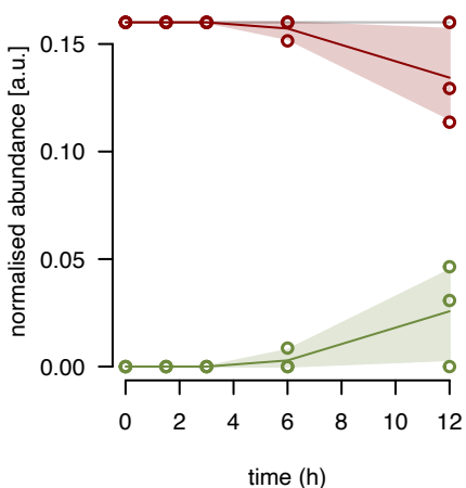
uL2m fraction 13
