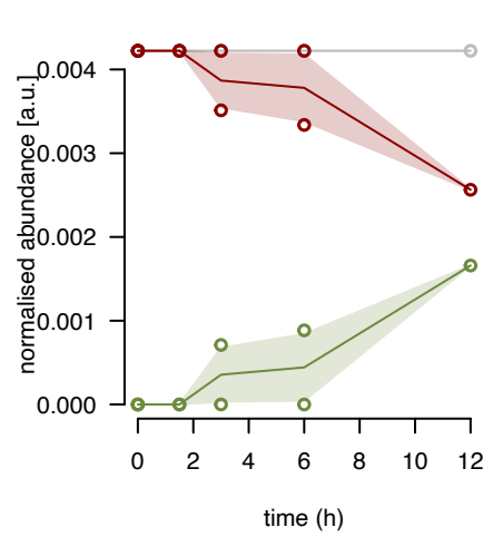
bL17m fraction 7
