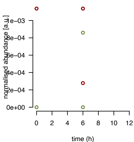
mL45 fraction 6
