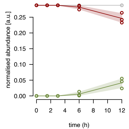
uL29m fraction 12
