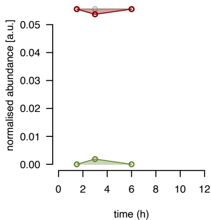
mL63 fraction 7
