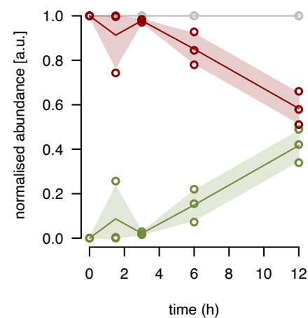
bL21m fraction 8
