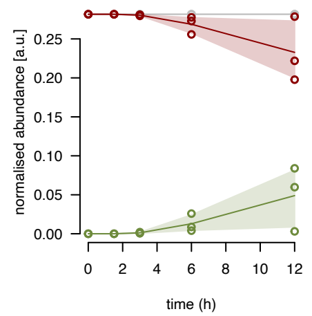
uL4m fraction 12
