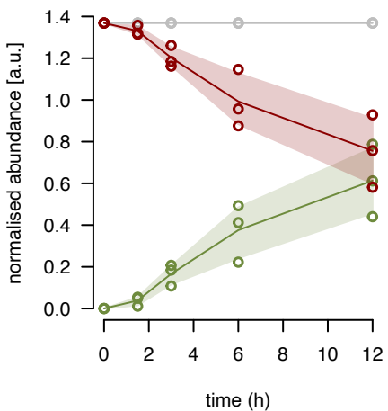
mL62 fraction 9
