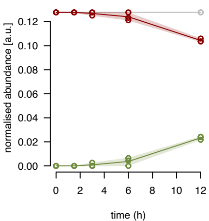
mL38 fraction 13
