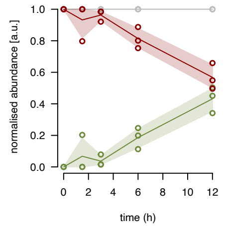
uL4m fraction 8
