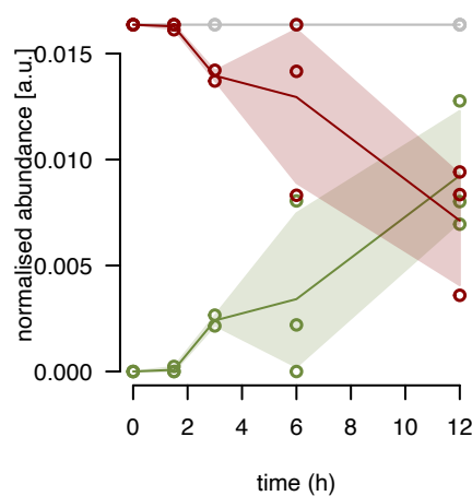
bL21m fraction 7
