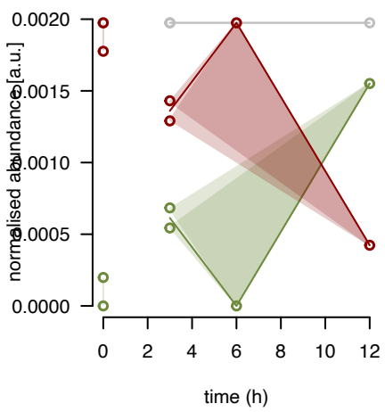
bL19m fraction 5
