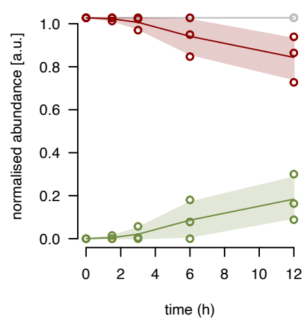
mL62 fraction 16
