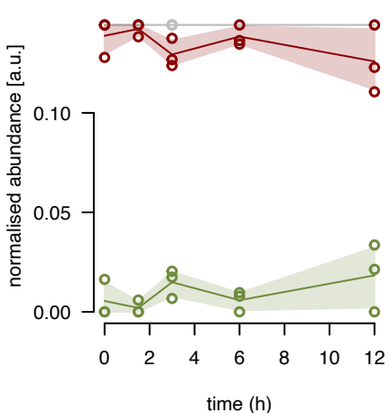
mL45 fraction 13
