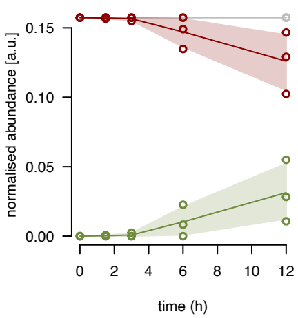
bL19m fraction 13
