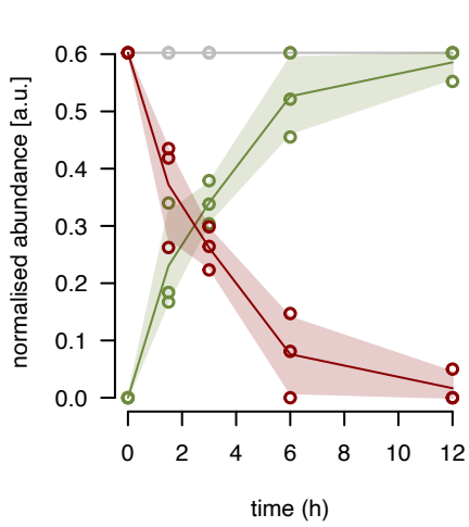
mL39 fraction 2
