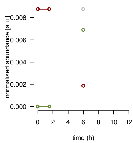
uL1m fraction 3
