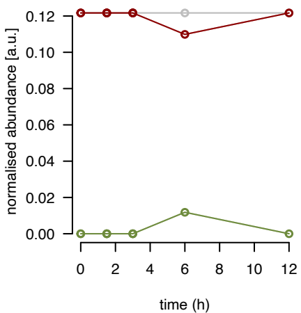
mL51 fraction 13
