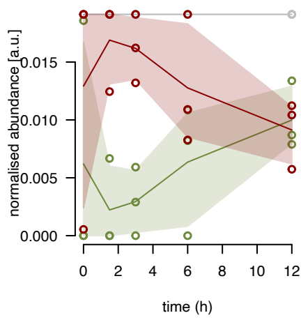
uL22m fraction 6
