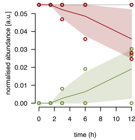
uL10m fraction 7
