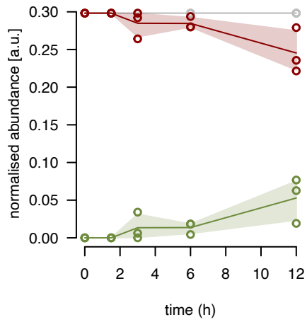
uL10m fraction 14
