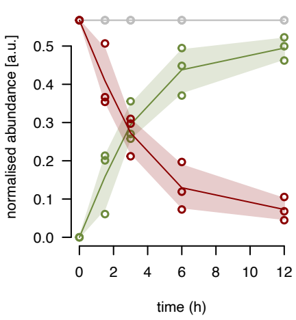
uL14m fraction 1
