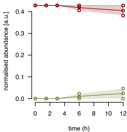
mL63 fraction 11
