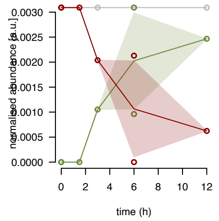
mL38 fraction 8
