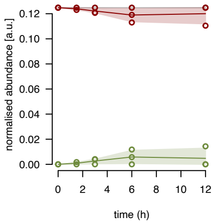
mL41 fraction 14
