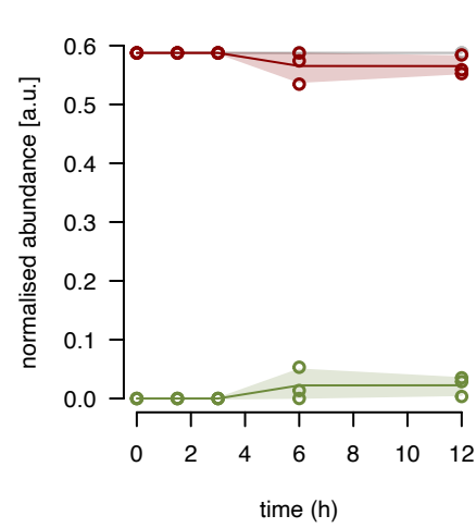
mL40 fraction 12
