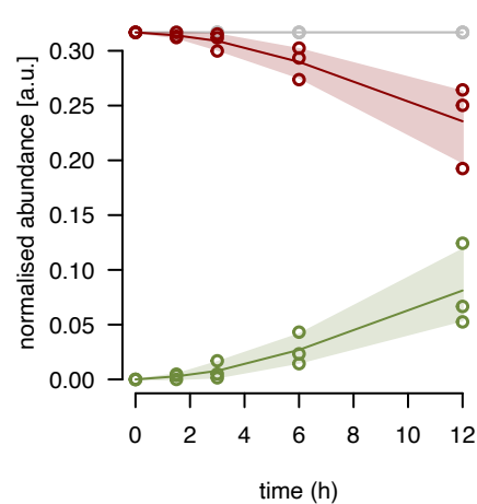
uL3m fraction 12
