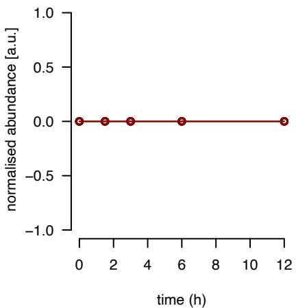
mL63 fraction 1
