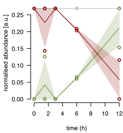
uL1m fraction 2
