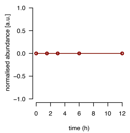
uL30m fraction 4
