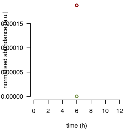
mL63 fraction 6
