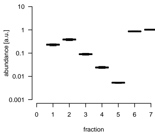
abundances
