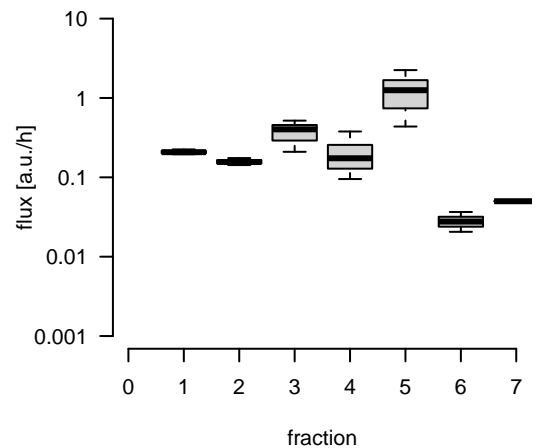
fluxes
