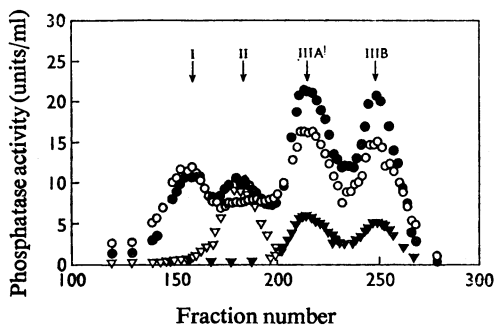
Fig. 5. Elution profile of histone phosphatases from a column (150 cm \times 2.5 cm) of Sephadex G-200. Fractions from the column shown in Fig. 3 were analysed for histone phosphatase activity with the following substrates: \circ , histone H1 containing 0.72 mol of phosphate per mol; \bullet , histone H2B containing 1.83 mol of phosphate per mol. Phosphorylase phosphatase ( \nabla ) and \alpha -phosphorylase kinase phosphatase ( \nabla ) activities are also shown. The substrates used to assay these activities are described in Fig. 3. \beta -Phosphorylase kinase phosphatase activity is omitted.
