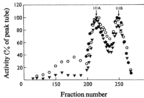
Fig. 3. Elution profile from a column (150 cm \times 2.5 cm) of Sephadex G-200 showing equal amounts of peaks IIIA and IIIB
