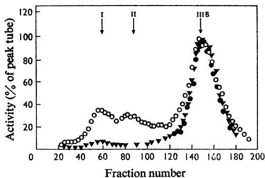
Fig. 4. Elution profile from a column (150 cm \times 2.5 cm) of Sephadex G-200 showing predominantly peak IIIB. A sample (4.0 ml) was applied to the column and 4.4 ml fractions were collected. Other conditions are as in Fig. 3. The fractions were assayed with: \nabla , phosphorylase a containing 0.91 mol of phosphate per subunit; \circ , glycogen synthase b 1 containing 1.09 mol of phosphate per subunit; \bullet , phosphorylase kinase containing 0.7 mol of phosphate in the \alpha -subunit and 1.0 mol in the \beta -subunit. Only \beta -phosphorylase kinase phosphatase activity is illustrated.
