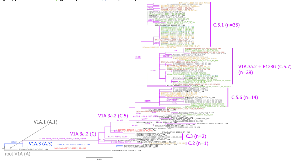
Supplemental Figure 2 S2. Phylogenetic comparison of influenza B/Victoria-lineage haemagglutinin genes. The vaccine strains are red, reference strains black and sequences reported to TESSy coloured according to the virus collection date by month (2023: October red, November yellow, December grey; 2024: January green, February, turquoise).
