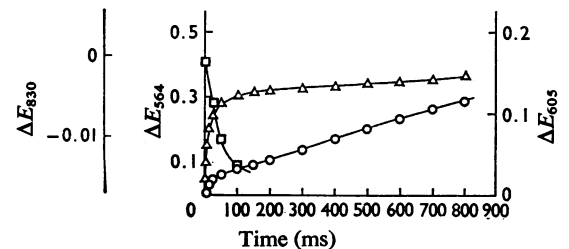
Fig. 5. Oxidation of ferrocytochrome c by cytochrome oxidase in the presence of a low oxygen concentration
