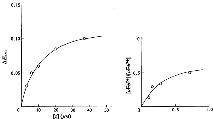
Fig. 8. 'Burst'-phase oxidation of ferrocyanochrome by cytochrome oxidase
