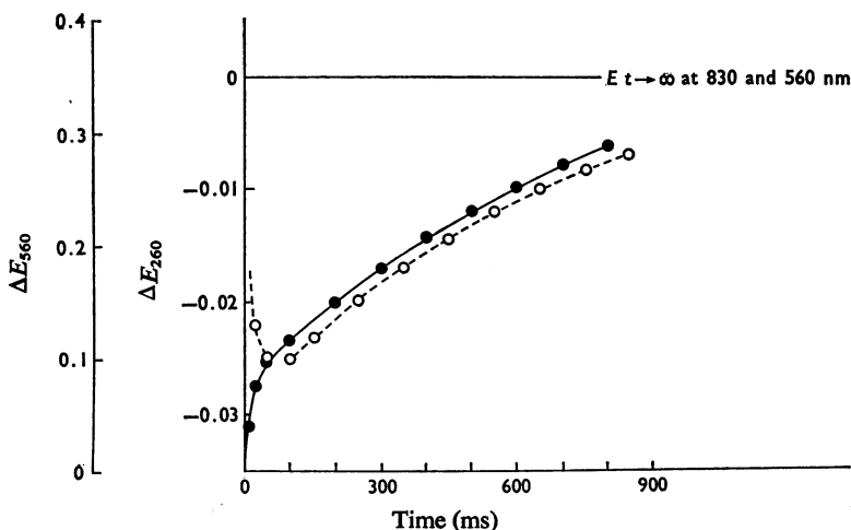
Fig. 9. Aerobic oxidation of ferrocytochrome c by cytochrome oxidase
