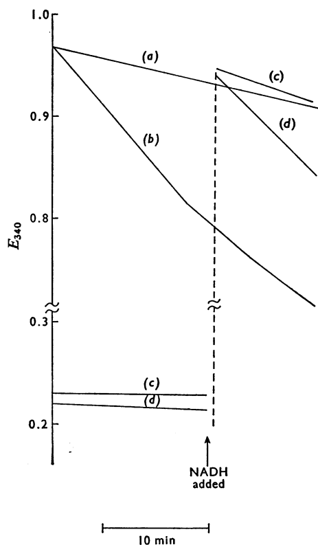
Fig. 2. Effect of time of addition of NADH on the stimulation by glutamine of the oxidation rate in the presence of \alpha -oxoglutarate
