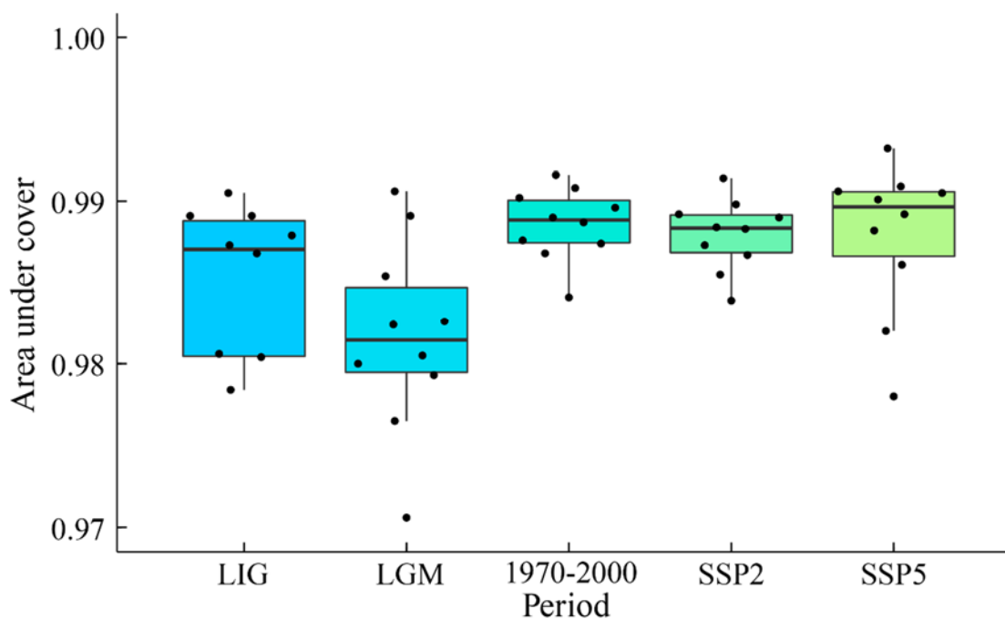
Fig. S4. Precision evaluation of MaxEnt model for the five periods. Model accuracy was assessed by 10-fold cross-validation. All models' mean AUC_{TEST} values are greater than required for a significant threshold of the random prediction (0.5), implying the modeled predictions are "excellent." As for LIG and LGM, the mean AUC_{TEST} is 0.983 \pm 0.010 and 0.982 \pm 0.006 , respectively. The same values are 0.989 \pm 0.002 for 1970-2000; 0.988 \pm 0.002 for SSP2; and 0.988 \pm 0.004 for SSP5.
