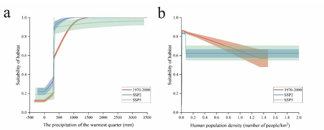
Fig. S6. Response curve of the precipitation of the warmest quarter (var8) and the human population density (var16).
