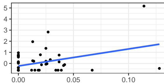
LPA, Megestrol acetate
