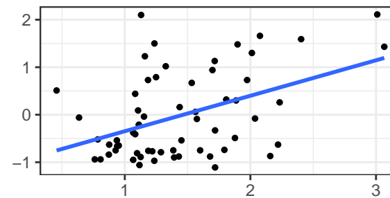
EMP1, Nitrogen mustard
