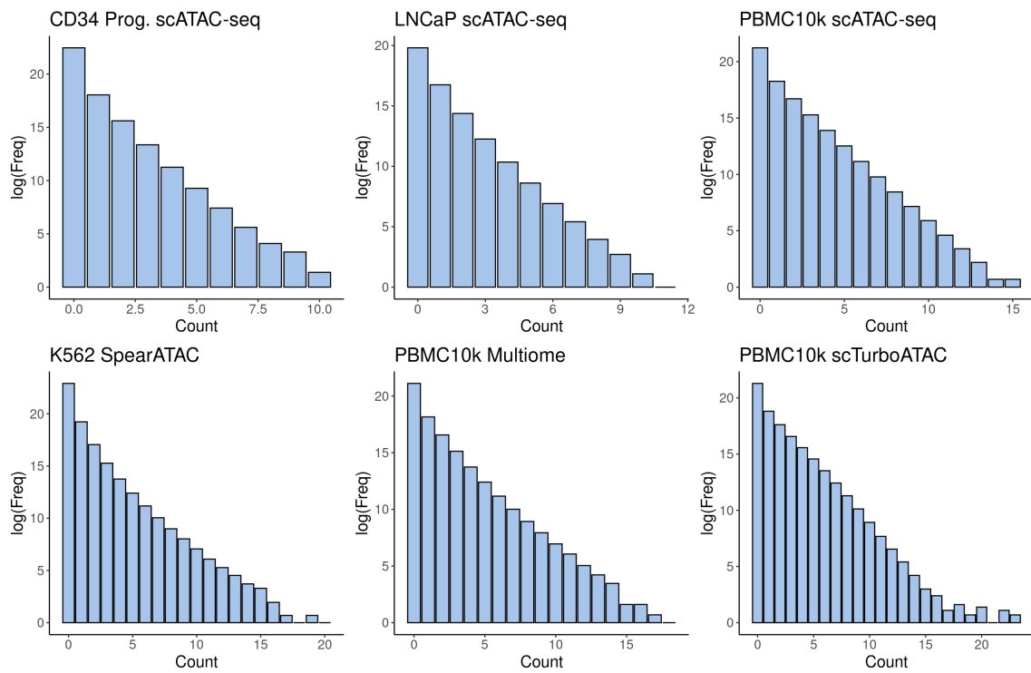
Figure S1: Histogram of paired-insertion counts (PIC) for all datasets analysed.
