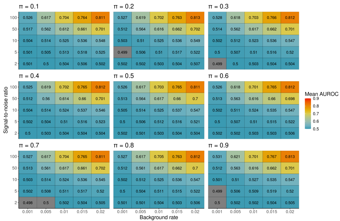
Figure S2: Simulations with varying \pi .
