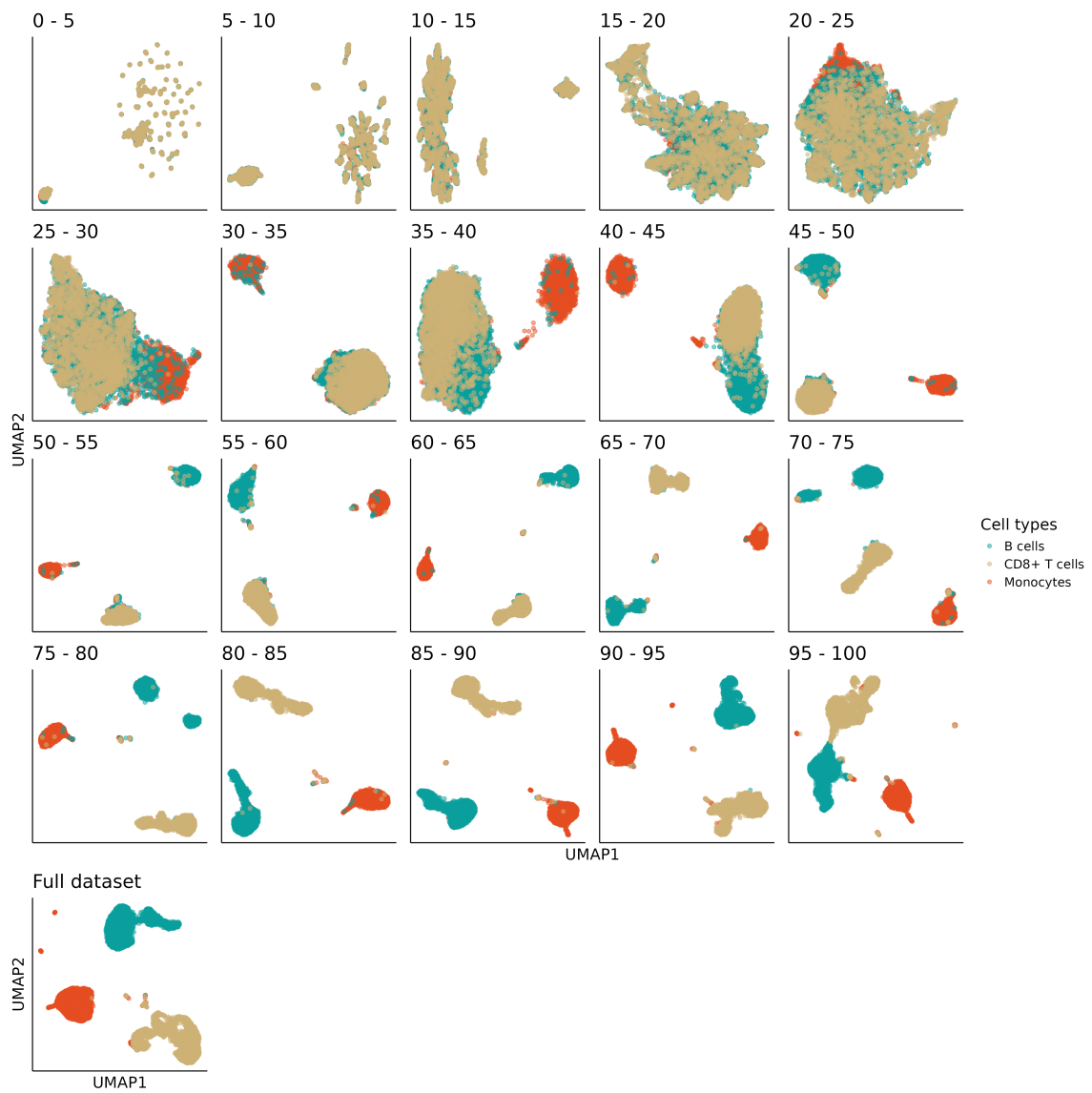
Figure S3: UMAPs of clustering with varying peak quantiles.
