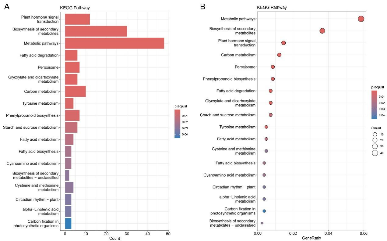
Supplementary Figure 2. KEGG pathway enrichment analysis of DEGs. (A) Bar plot of significantly enriched KEGG pathways for all DEGs. (B) Dot plot of significantly enriched KEGG pathways for all DEGs
