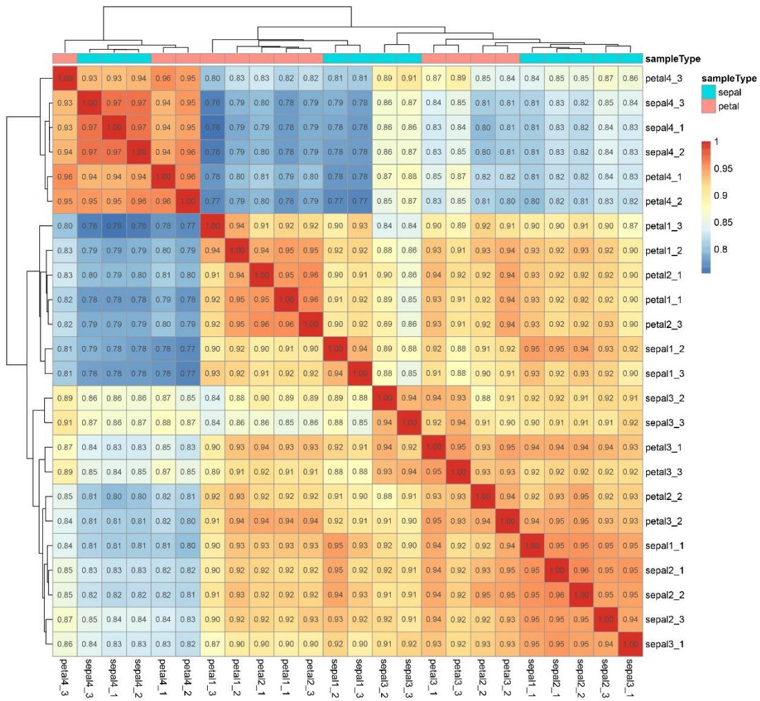
Supplementary Figure 1. Correlation of gene expression between RNA-seq samples.
