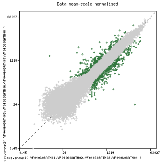
4 cad-c cad-d ATH1 genechips versus 4 wild-type ATH1 genechips
