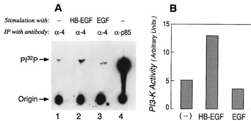
Fig. 9. Ligand-stimulated PI3-K activity. (A) Cells expressing HER4 were stimulated without (lanes 1 and 4) or with 100 ng/ml of HB-EGF (lane 2) or with 100 ng/ml of EGF (lane 3). The cells were lysed and aliquots from the lysates were immunoprecipitated with polyclonal anti-HER4 antibodies (lanes 1–3) or with monoclonal anti-p85 antibodies (lane 4). The co-precipitated material was analyzed for PI3-K activity using an in vitro kinase assay that measures incorporation of 32 P into [ 32 P]PI using TLC. The positions of [ 32 P]PI and the origin of the chromatography are indicated. (B) The amount of [ 32 P]PI associated with the TLC membrane shown in (A) was quantitated using a PhosphorImager (Molecular Dynamics).
