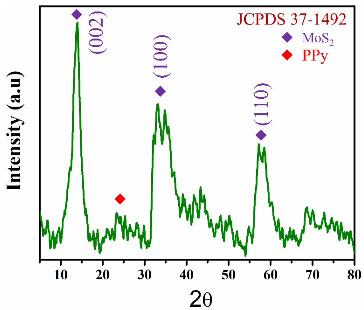
Fig. 1 XRD of PPy/MoS 2
