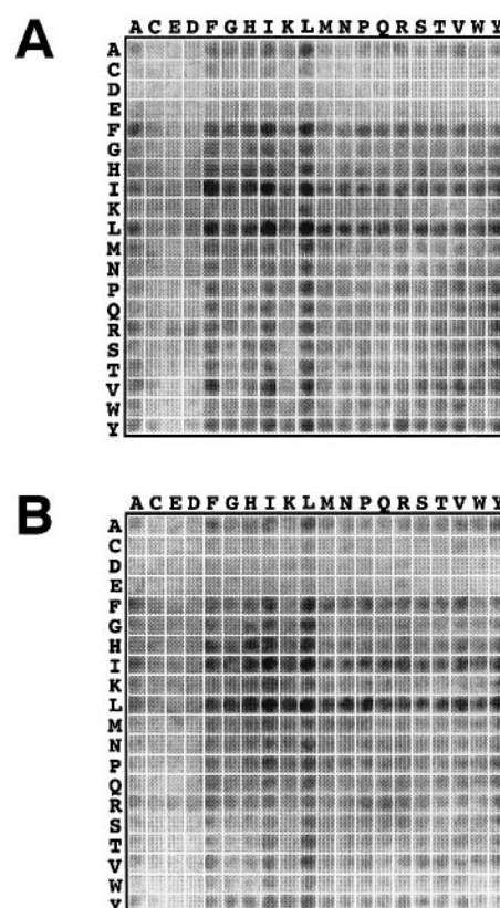
Fig. 4. DnaK binding to combinatorial peptide libraries X 5 B 1 XB 2 X 5 (A) and X 5 B 1 XXB 2 X 4 (B). B 1 (rows) and B 2 (columns), defined positions; X, randomized positions (19 amino acids, Cys omitted) (Kramer et al. , 1994; Kramer and Schneider-Mergener, 1997).
