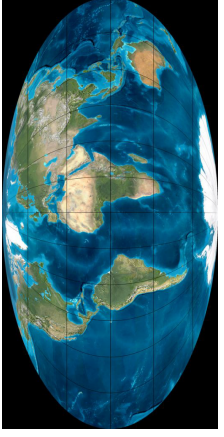
now
