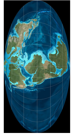
150 Mya
