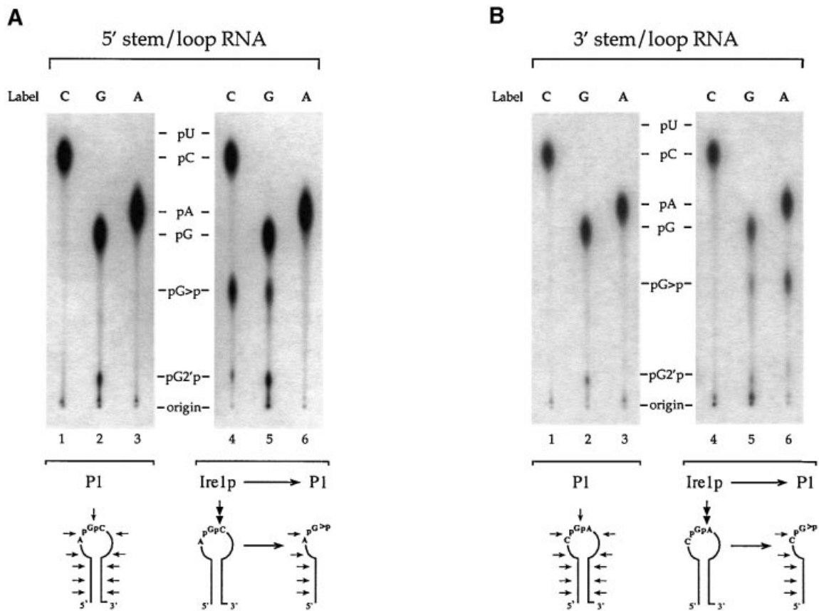
Fig. 4. Formation of 3' terminal guanosine 2',3'-cyclic phosphate after Ire1p(k+t) cleavage of stem-loop RNA. 5' stem-loop RNA ( A ) or 3' stem-loop RNA ( B ) was labeled with [\alpha\text{-}^{32}\text{P}]\text{CTP} (lanes 1 and 4), [\alpha\text{-}^{32}\text{P}]\text{GTP} (lanes 2 and 5) or [\alpha\text{-}^{32}\text{P}]\text{ATP} (lanes 3 and 6). The labeled RNAs were then digested with P1 nuclease (lanes 1–3). Alternatively, they were first digested (40 000 to 60 000 c.p.m. of each stem-loop RNA) with Ire1p(k+t). The 5' cleavage product was then isolated by preparative gel electrophoresis and digested with P1 nuclease (lanes 4–6). The final digestion products were separated by TLC on PEI cellulose plates and visualized by autoradiography. The position of marker nucleotides on the thin layer plates are indicated, where pG>p refers to a G bearing a 5' phosphate and a 2',3'-cyclic phosphate. Digestion of the relevant portions of the stem-loop structures is indicated schematically below each panel. The ratios of labeled pG>p relative to labeled pN were determined and are in good agreement with the expected values. ( A ) Lanes 4 and 5: pC/pG>p expected = 0.25, actual = 0.26; pG/pG>p expected = 0.13, actual = 0.18. ( B ) Lanes 5 and 6: pG/pG>p expected = 0.17, actual = 0.21; pA/pG>p expected = 0.25, actual = 0.26. Note also that a variant of the wild-type 5' stem-loop was used in this analysis (hactng-39). In this stem-loop, a GC dinucleotide pair in the stem was changed, leaving the only GC dinucleotide in the loop. The only GA dinucleotide in the wild-type 3' stem-loop (hactng-10) was in the loop.
