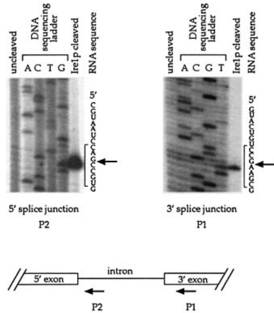
Fig. 6. Ire1p(k+t) cleaves HAC1 u RNA at the same positions as it cleaves the 5' and 3' stem-loops. Primer extension analysis was performed on both undigested and Ire1p(k+t)-digested HAC1 u 508 RNA using 5' end-labeled DNA primers. HAC1 u 508 RNA consists of a truncated 5' exon (181 nucleotides), an intact HAC1 u intron (252 nucleotides), and a truncated 3' exon (75 nucleotides), as previously described (Sidrauski and Walter, 1997). Extensions on uncleaved RNA served as controls for natural pausing during the extension reaction. The Ire1p(k+t) cleavage site is indicated by an arrow along side the RNA sequence corresponding to the DNA ladder; the residues in the 7-membered loop are marked with a bracket.
