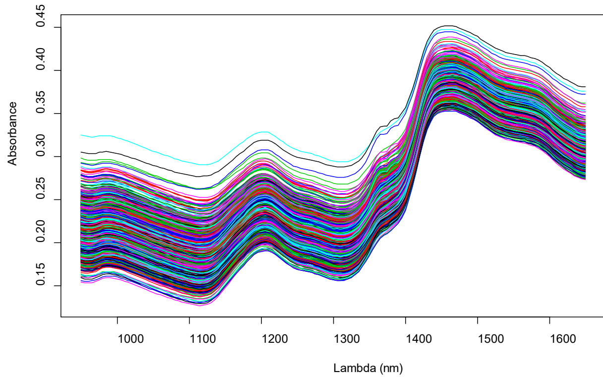
Figure S1. Change in absorbance from 950 to 1650 nm for raw NIR wavelengths (lines with different colors) for whole barley grain after malting.
