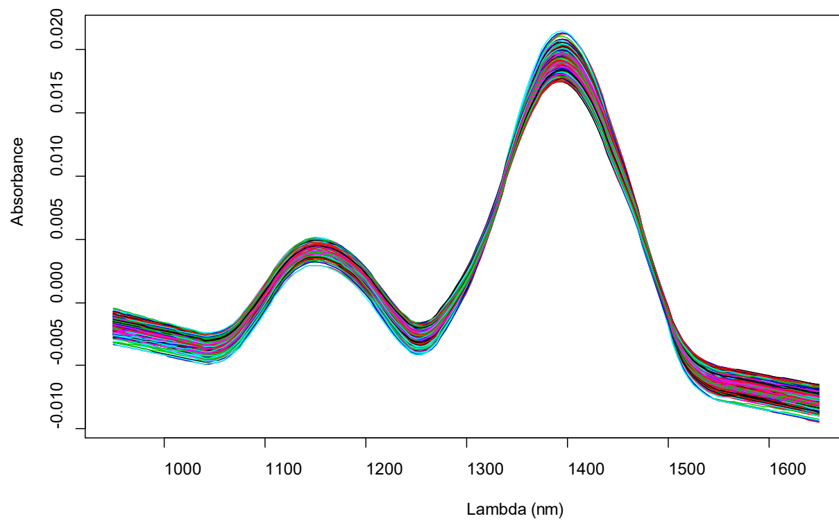
Figure S2. Change in absorbance from 950 to 1650 nm for NIR wavelengths after Savitzky-Golay transformation (lines with different colors) for whole barley grain after malting.
