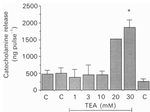
Fig. 8. Effects of tetraethylammonium (TEA) on the release of catecholamines evoked by methacholine pulses ( 100 \mu\text{M} for 10 s) given at 15 min intervals. The initial rate of methacholine-evoked secretion is indicated by the first two columns (C, control secretion). Each concentration of TEA was present 5 min before, during the methacholine pulse and during the post-stimulation sample collection. At the end of the experiment, a new control test stimulus was applied in order to see the reversibility of the TEA effects. Data are means \pm s.e.m. of three glands; the datum for the 20 mM-TEA concentration is from a single gland. * P < 0.01 with respect to the initial controls.
