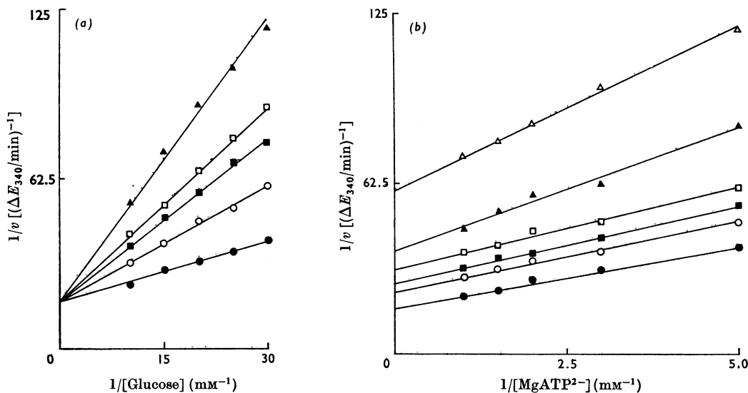
Fig. 3. N -Acetylglucosamine inhibition of cerebral mitochondrial hexokinase. (a) Plot of 1/v versus 1/[\text{glucose}] at a constant concentration of 0.5mM- \text{MgATP}^{2-} and N -acetylglucosamine concentrations of: \blacktriangle , 1.0mM; \square , 0.50mM; \blacksquare , 0.33mM; \circ , 0.20mM; \bullet , nil. (b) Plot of 1/v versus 1/[\text{MgATP}^{2-}] at constant 0.10mM-glucose and N -acetylglucosamine concentrations of: \triangle , 2.0mM; \blacktriangle , 1.0mM; \square , 0.5mM; \blacksquare , 0.33mM; \circ , 0.2mM; \bullet , nil. Experimental details are described in the Materials and Methods section.
