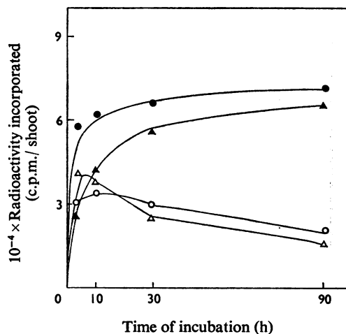
Fig. 4. Incorporation of radioactivity from [ ^{14}\text{C} ]methylamine into \gamma -glutamylmethylamide ( \bullet ), serine ( \circ ), theobromine ( \Delta ) and caffeine ( \blacktriangle ) in tea shoot tips
