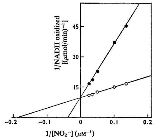
Fig. 2. Competitive inhibition by cyanide with respect to nitrite of A. chroococcum nitrite reductase activity. Experimental conditions were as in the standard assay for NADH–nitrite reductase activity, except that nitrite was added as indicated. ●, + Cyanide (0.125 μM); ○, control, no cyanide. Enzyme preparation, 0.6 mg.
