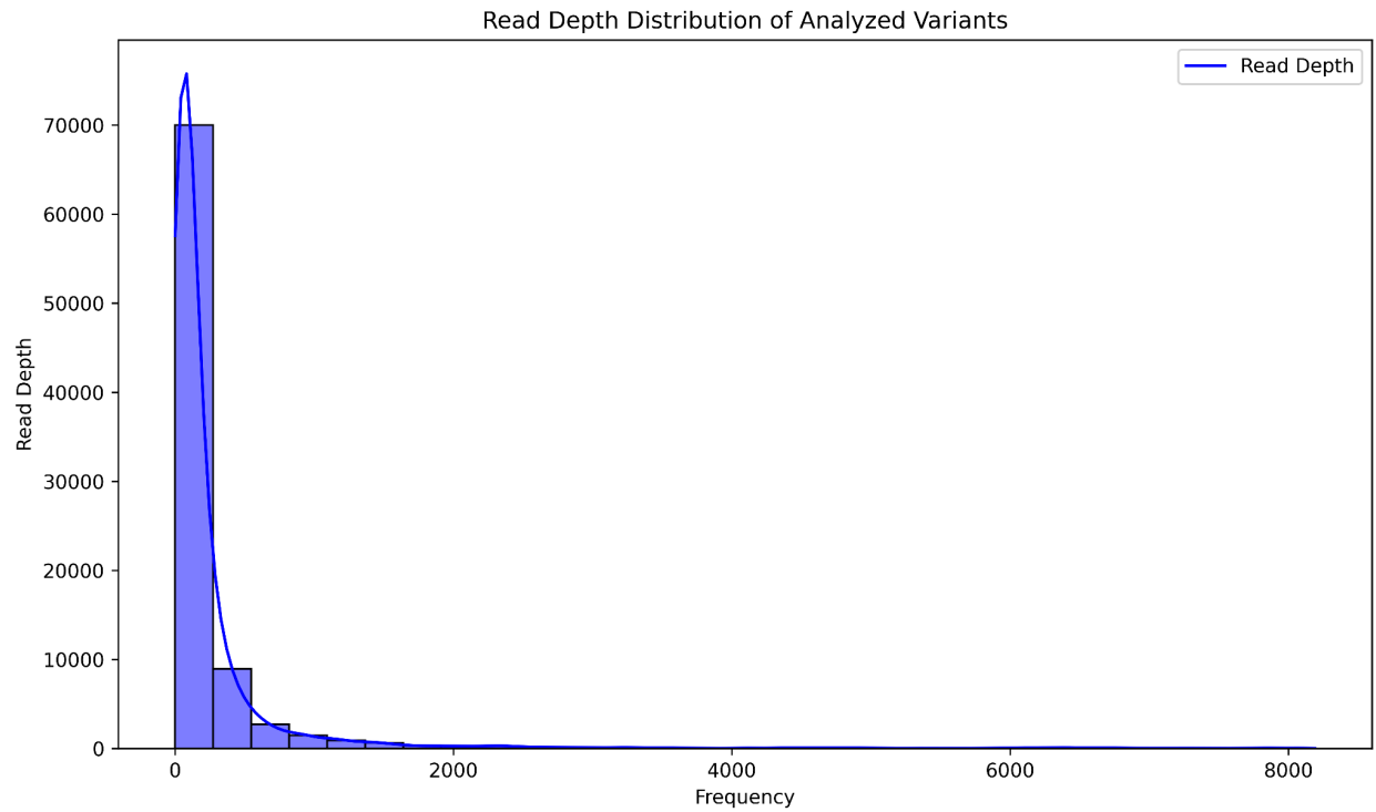
Supplementary Figure 2 - Distribution of Read Counts for Heterozygous Loci : The distribution of read depth for each of the loci used in this study's analysis
