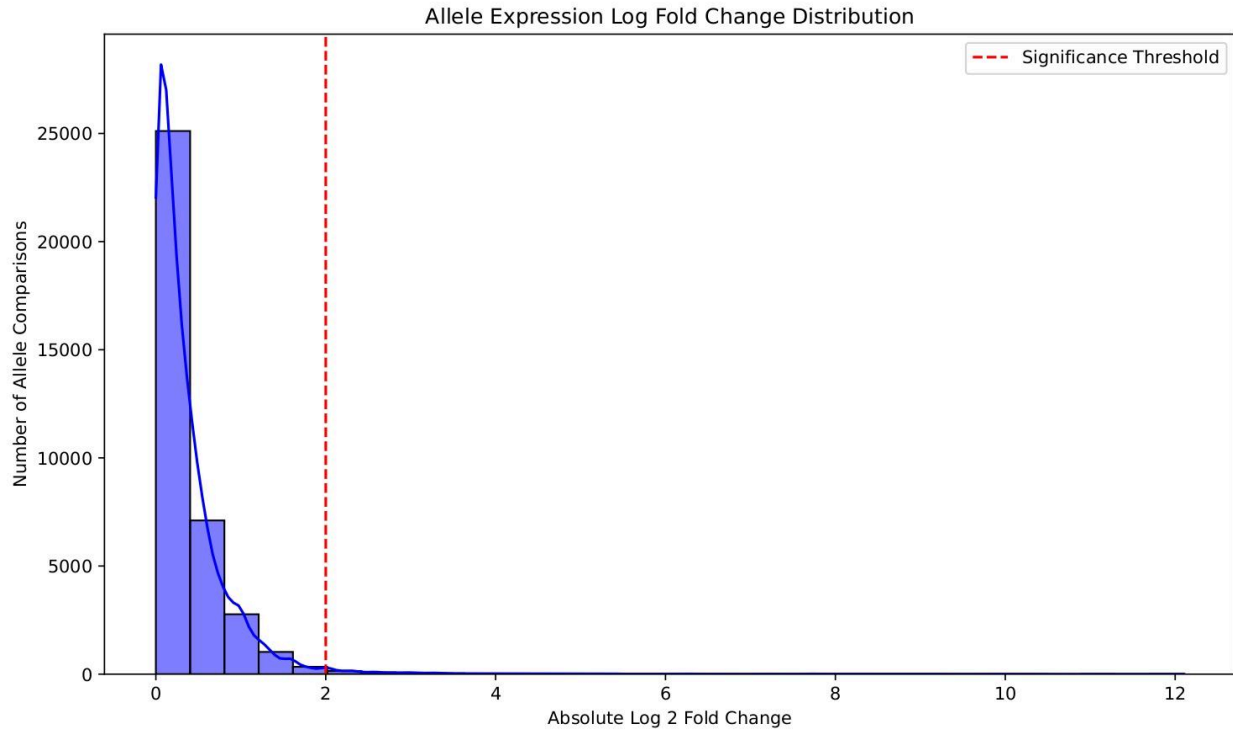
Supplementary Figure 3 - Distribution of Allele Expression Fold Change for All Allele Comparisons : The distribution of the allele expression fold changes for all of the loci analyzed in this study. The red dotted line represents the Allele expression fold change threshold for declaring a haplotype as potentially having a significant preference for being transcribed.
