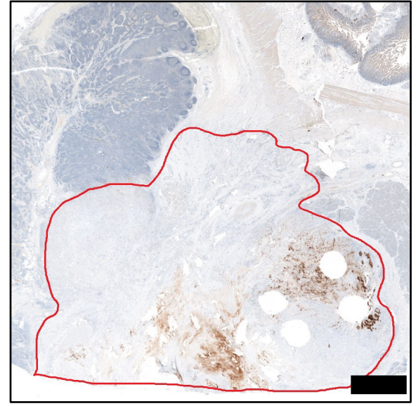
Whole slide
