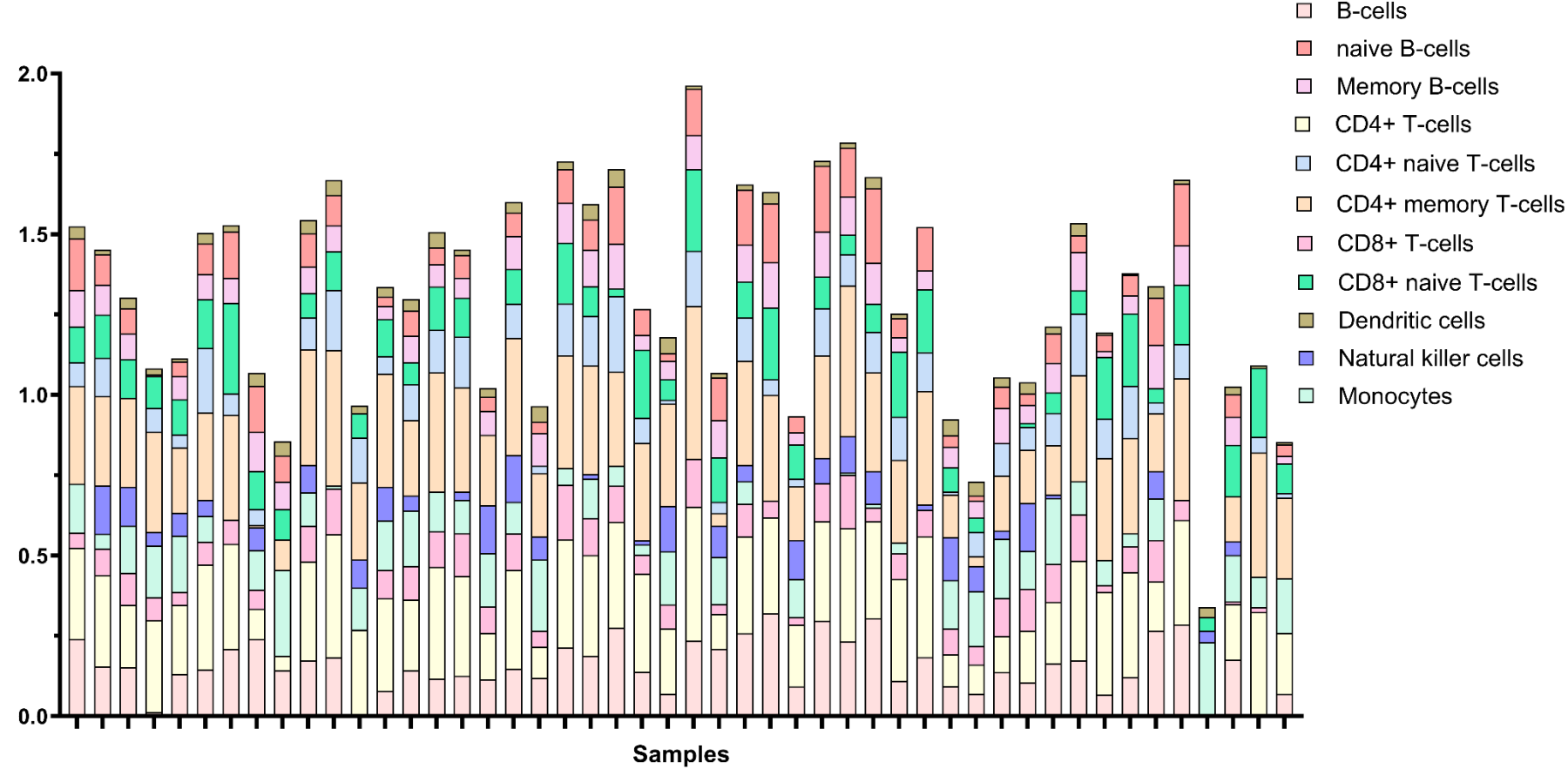
Supplementary Figure 1. Visualization of xCell scores for each of the major PBMC cell types estimated by the xCell algorithm in baseline samples.
