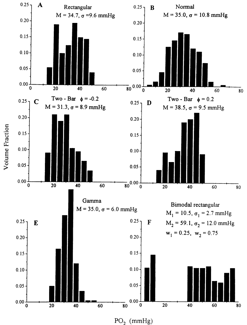
FIGURE 2 Computer-generated distributions of quencher concentration. Monte Carlo simulations were made by dividing the excitation volume into 200 regions of equal size and randomly drawing an oxygen tension (PO 2 ) from a specified continuous distribution with mean PO 2 of 35 mmHg and standard deviation of 10 mmHg.
