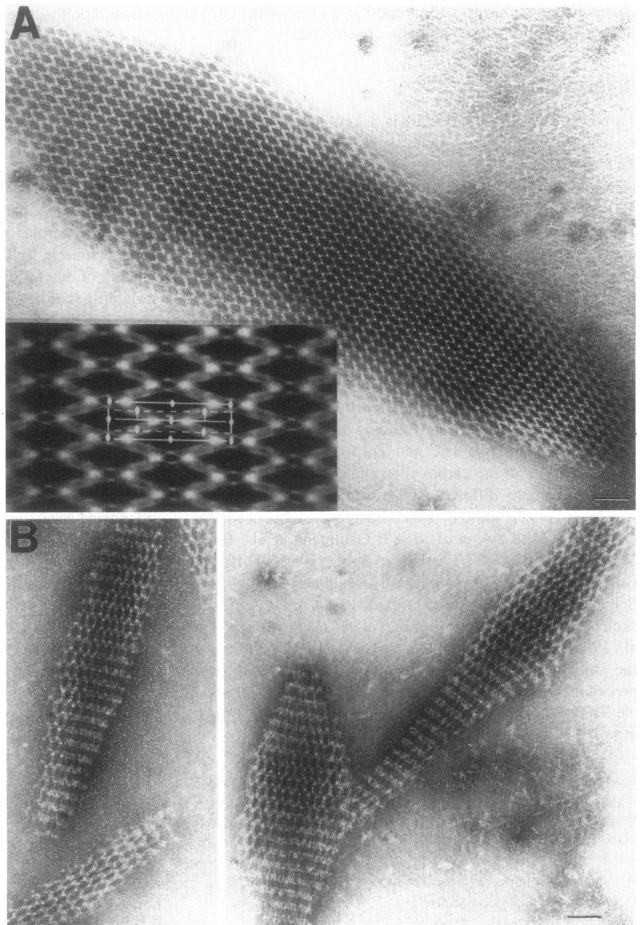
FIGURE 1 Electron micrographs of double diamond co-crystals of tropomyosin-TnT specimens in negative stain. Protein appears as white on a black background. The open-mesh pattern in the images collapses at one end into the double-ladder tactoid observed by others for these crystals (Cohen et al., 1972; Carr et al., 1988). (A) Image of a double diamond crystal of rabbit \alpha_2 -tropomyosin and rabbit skeletal TnT negatively stained with uranyl acetate. Bar, 100 nm. The inset shows a noise-filtered image of a selected portion enlarged approximately three times. An area of the lattice outlining the double-diamond pattern is shown ( thin white lines ) with one unit cell ( thick white lines ) and associated symmetry elements. The projection (viewed down c ) has cmm plane group symmetry with a = \sim 726 Å and b = \sim 324 Å. (B) Electron micrographs of representative tropomyosin-TnT trunc co-crystals. Bar, 100 nm.
