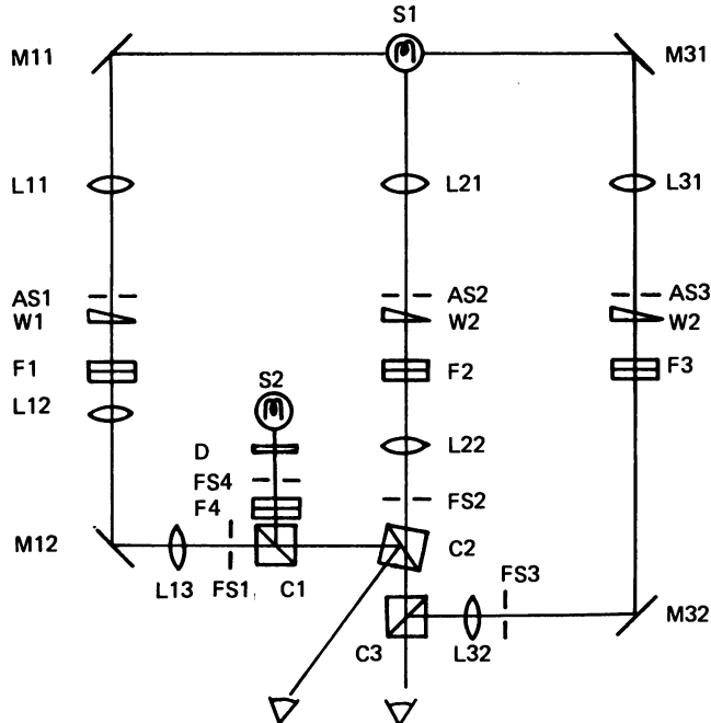
Fig. 3. Schematic diagram of optical apparatus. See text for abbreviations and details.
