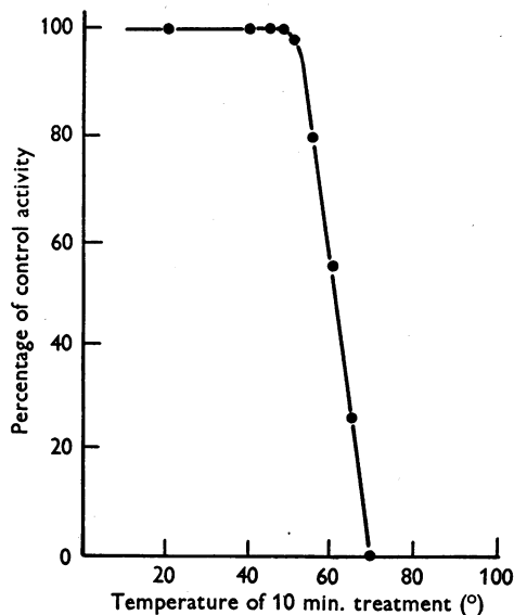
Fig. 7. Thermal inactivation of phytase in solution (705 units/ml.). Activities of samples of a partially purified solution of phytase heated to various temperatures in sealed ampoules for 10 min., determined in buffered substrate, pH 5.15, at 55°.
