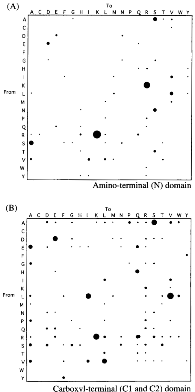
FIGURE 5.—The average frequency of different amino acid replacements for (A) the N domain (96–272 in consensus) and (B) the C1 and C2 domains (273–348, 418–456). Ancestral states were inferred by using the MacClade program (MADDISON and MADDISON 1992). The diameter of the largest circle in A is proportional to nine changes, and other circles in A and B are scaled in diameter proportionally.
