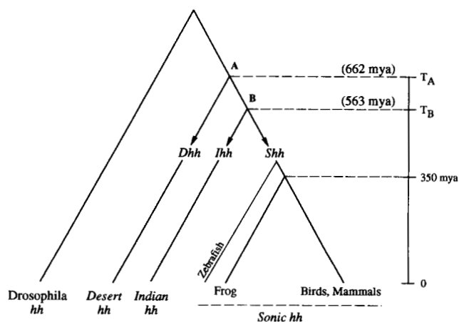
FIGURE 4.—Model for the evolution of the hedgehog gene family. The approximate times of the gene duplication events at nodes A and B in Figure 2 were computed by equation (4). The standard errors of the estimates of T_A and T_B are of the order of 100 mya.
