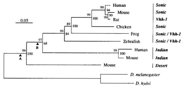
FIGURE 2.—Evolutionary relationships of genes of the hedgehog family. The NJ method based on d -distance with the complete-deletion option in MEGA (KUMAR et al. 1993) program was used. Only N and C domains sequences (96–526) were used. Results from the interior branch length test (confidence probability that a branch length is significantly different from 0) are shown above the corresponding branches, and the numbers to the right of each fork represent the percentage of the bootstrap replicates that support the branch. The scale bar has the units of number of amino acid replacements per site. In the maximum parsimony branch-and-bound analysis, a single most parsimonious tree was recovered, which was identical in topology to the NJ tree.
