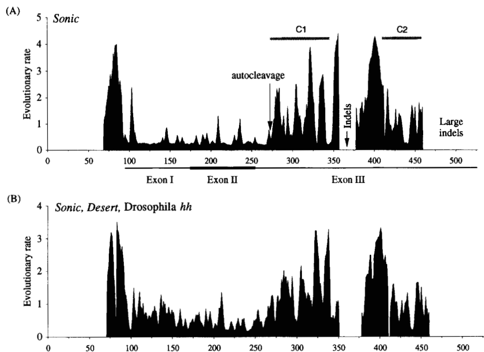
FIGURE 3.—The number of amino acid replacements per site (A) in only Shh genes and (B) in all hh genes except Ihh , which was excluded because the sequence of the first exon was not available at the time of the analysis. The rate of amino acid substitution at each site were determined by the maximum-likelihood approach and the moving average in segments of length 5 were plotted at the center of each segment (see text for details). Sites are numbered following the consensus sequence in Figure 1. Regions with extensive alignment gaps or missing data are marked as indel regions. Various landmarks shown in Figure 1 are also marked.
