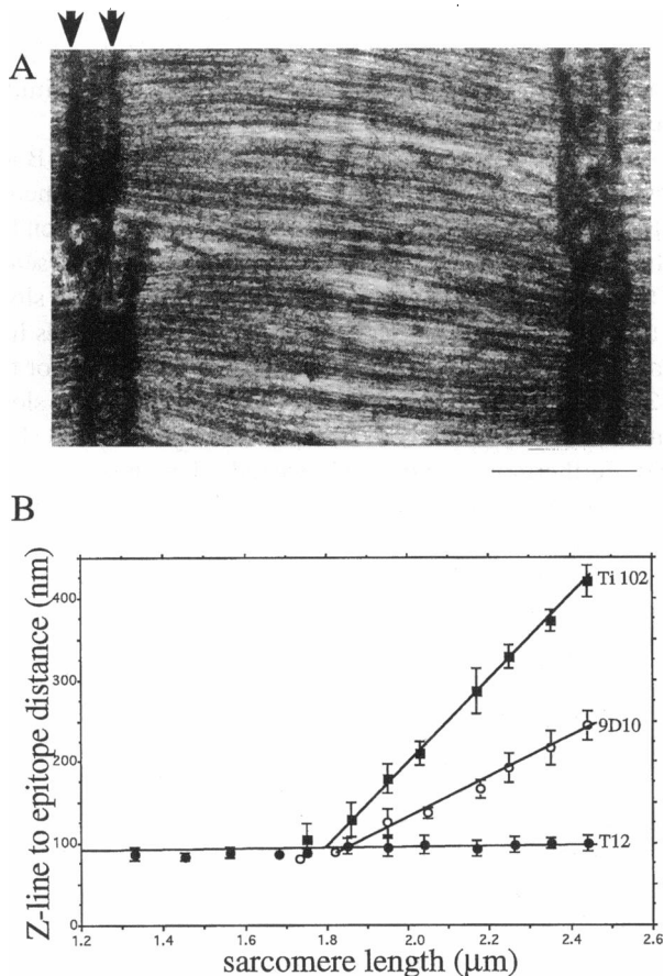
FIGURE 6 Titin behavior in short sarcomeres. (A) Short sarcomere ( \sim 1.7 \mu\text{m} ) labeled with T12, 9D10, and Ti-102. No separate epitopes can be seen. Instead, a single dark stripe is present in each I-band (arrows), approximately 100 nm from the center of the Z-line. Scale bar, 0.5 \mu\text{m} . (B) Sarcomere length dependence of distance between the Z-line and T12 ( \bullet ), the Z-line and 9D10 ( \circ ), and the Z-line and Ti-102 ( \blacksquare ). Epitopes converge at a sarcomere length of \sim 1.8 \mu\text{m} . See text for further details. For clarity's sake, results were grouped in sarcomere length bins of 0.1 \mu\text{m} . Mean values \pm SDs are shown for distances. For sarcomere length, the mean value of all data in the bin is given. (Note that thick filaments in A are slightly bent, despite that the sarcomere is longer than the A-band width. Bending may result from a compressive force exerted by titin when sarcomeres shorten below the slack length. See Discussion and Fig. 9.)
