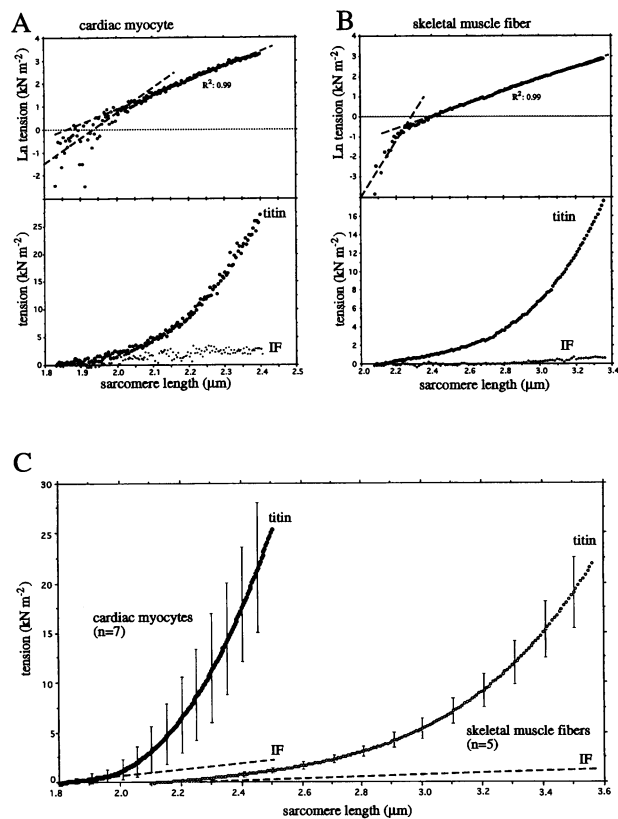
FIGURE 7 Passive tension-sarcomere length relations of rat cardiac myocytes and rabbit skeletal muscle fibers (semitendinosus). (A and B, bottom panels) Sarcomere length dependence of KCl/KI-sensitive tension (titin) and KCl/KI-insensitive tension (IFs). Titin-based tension is much larger than IF-based tension. (A and B, top panels) Natural logarithm of titin-based tension versus sarcomere length. Results of cardiac myocytes at lengths <2.0 \mu\text{m} and those at lengths >2.0 \mu\text{m} were fitted by two straight lines. The 95% confidence intervals of the slopes of these lines were 7.1–14.7 and 6.2–6.5, respectively. Results of skeletal muscle fibers at lengths <2.3 \mu\text{m} and at >2.3 \mu\text{m} were also fitted by two separate straight lines, and their 95% confidence slope intervals were 10.8–16.6 and 3.0–3.1, respectively. (C) Comparison of titin-based and IF-based tensions from cardiac myocytes and skeletal muscle fibers. Results of seven myocytes and five skeletal muscle fibers were pooled, and their mean values and SDs are shown (for clarity's sake the SD is displayed for only some of the data points, whereas for IFs only a linear fit to the data is shown.) At a given sarcomere length, cardiac titin developed much higher passive tensions than skeletal muscle fibers did.
