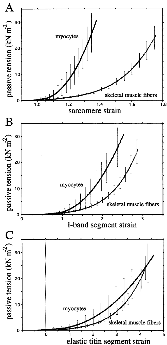
FIGURE 8 Dependence of titin-based passive tension on (A) sarcomere strain, (B) strain of total I-band segment of titin, and (C) strain of the elastic I-band segment of titin. Strain defined as L/L_0 . See Table 1 and text for further information. (Mean \pm SDs are shown. For clarity's sake the SD is displayed for only some of the data points. Same data as in Fig. 7 C.)
