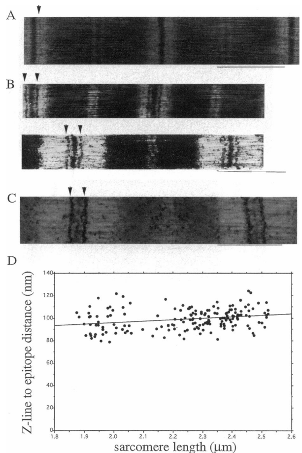
FIGURE 3 Sarcomere location of T12 titin epitope. (A) High magnification image of control sarcomeres (not labeled). The arrow indicates a faint line that can be seen in the I-band. (B) High magnification micrographs of sarcomeres labeled with T12 primary antibody and with secondary antibody. The upper panel shows a micrograph from a short sarcomere and the bottom panel a micrograph from a long sarcomere. In both sarcomeres, dense stripes on both sides of the Z-line can be seen (arrows). (C) Sarcomere labeled with T12 and with a nanogold-conjugated secondary antibody that was silver enhanced. Because the cell was not osmified, less structural detail can be seen than in A and B. Note the dark stripes (arrows) close to the Z-lines. Scale bars denote 1 μm. (D) sarcomere length dependence of distance between the T12 epitope and the center of the Z-line. The linear regression line fitted to the data is shown. See text for further details.
