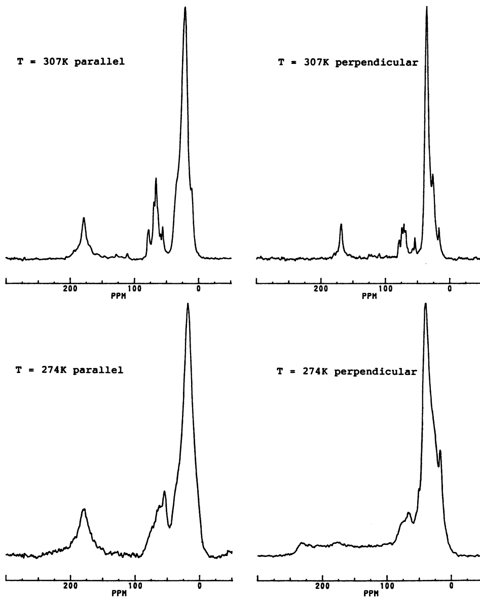
FIGURE 1 ^{13}\text{C} NMR spectra of GA13 at 75.48 MHz recorded above ( top ) and below ( bottom ) the lipid phase transition temperature for multilayers aligned with the bilayer normal parallel ( 0^\circ , left ) and perpendicular ( 90^\circ , right ) to the magnetic field direction. The spectra were processed with 100 Hz line-broadening. The peptide carbonyl resonances are near 175 ppm, and those further upfield are natural abundance signals arising from peptide and lipid.
