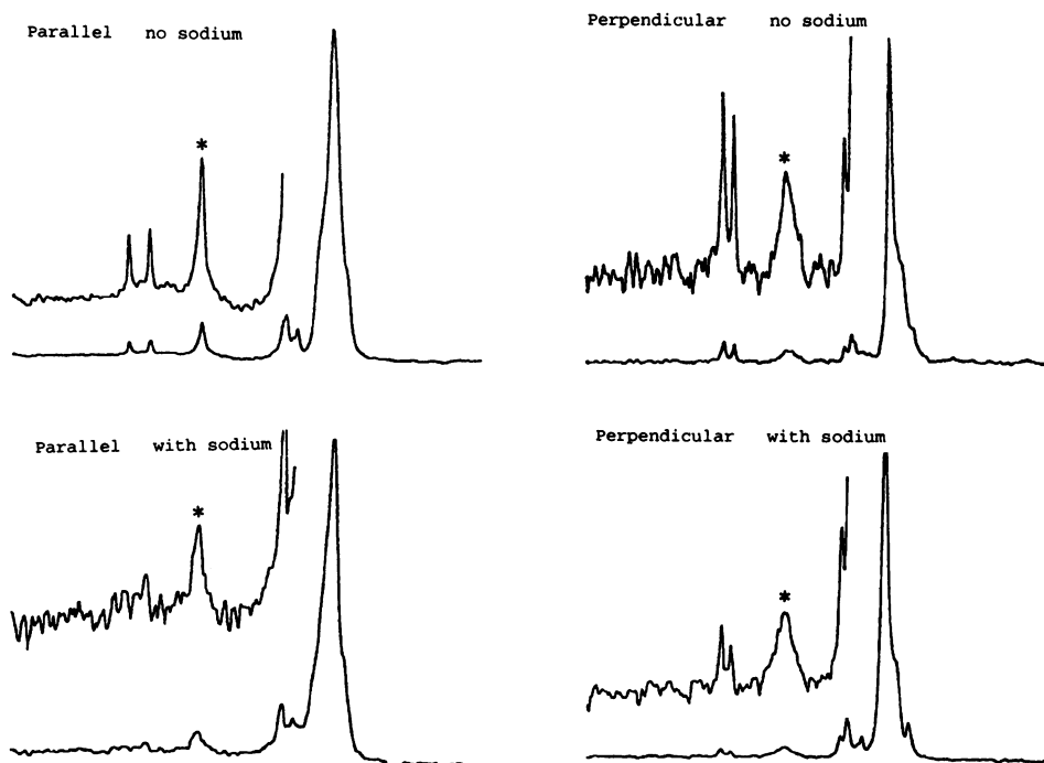
FIGURE 3 ^{13}\text{C} NMR spectra for Trp-15 [indole- 2\text{-}^{13}\text{C} ] gramicidin A at 0^\circ (left) and 90^\circ (right) to the magnetic field in DMPC at 307K with \text{Na}^+ (bottom) and without \text{Na}^+ (top) present. The plot width is 400 ppm. The indole resonance is marked with an asterisk in each spectrum; the other resonances are natural abundance signals arising from peptide and lipid.
