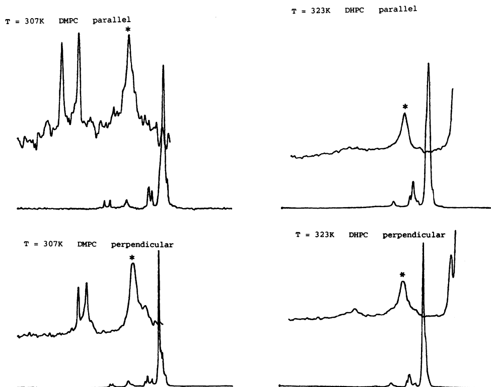
FIGURE 2 ^{13}\text{C} NMR spectra for Trp-11 [indole- 2\text{-}^{13}\text{C} ] gramicidin A at 0^\circ (top) and 90^\circ (bottom) to the magnetic field, in DMPC at 307 K (left; similar spectra were obtained at 323 K), and DHPC at 323 K (right). The plot width is 600 ppm, with the magnified region expanded by a factor of three. The indole resonance is marked with an asterisk in each spectrum; the other resonances are natural abundance signals arising from peptide and lipid.
