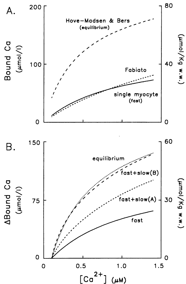
FIGURE 7 Comparison of intrinsic cytosolic Ca^{2+} buffers with published data. (A) Calculated bound Ca^{2+} is plotted against [Ca^{2+}]_i using the mean K_D and B_{max} for intrinsic cytosolic buffering in Table 1 (single myocyte), K_D and B_{max} values from Hove-Madsen and Bers (1993), and the sum of cytosolic Ca buffers listed in Table 2 of Fabiato (1983). (B) Calculated cytosolic buffers and the effect of slow Ca buffers. The change in bound Ca^{2+} from an initial level at 100 nM [Ca^{2+}]_i was calculated for the present data (fast) and that of Hove-Madsen and Bers (1993) (equilibrium). The curve labeled "fast + slow(A)" is that calculated by summing the change in Ca^{2+} binding predicted by the present data with that predicted for equilibrium Ca^{2+} binding to the Ca/Mg sites of troponin and myosin. The Ca^{2+} and Mg^{2+} affinities of the Ca/Mg sites are taken from Robertson et al. (1981). Myosin and troponin concentrations are taken from Fabiato (1983) assuming that myosin and troponin exist in a 1:1 ratio in the cytosol and that the molar ratio of Ca/Mg sites on cardiac troponin to Ca-specific sites is 2:1 (Robertson et al., 1981). The curve labeled "fast+slow(B)" is the same as "fast+slow(A)" except that the Mg^{2+} affinity of the Ca/Mg sites on troponin have been increased 10-fold.
