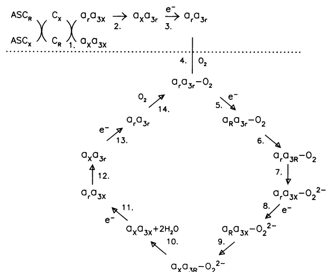
FIGURE 8 A model that can explain the observations made in these studies: The abbreviations ASC, C, and aa_3 , represent ascorbate, cytochrome c , and cytochrome aa_3 , respectively. The subscripts X, r, and R, represent the electron content of the individual center as 0, 1, and 2, respectively. The relation of this model to the experimental observations is discussed in the text.
