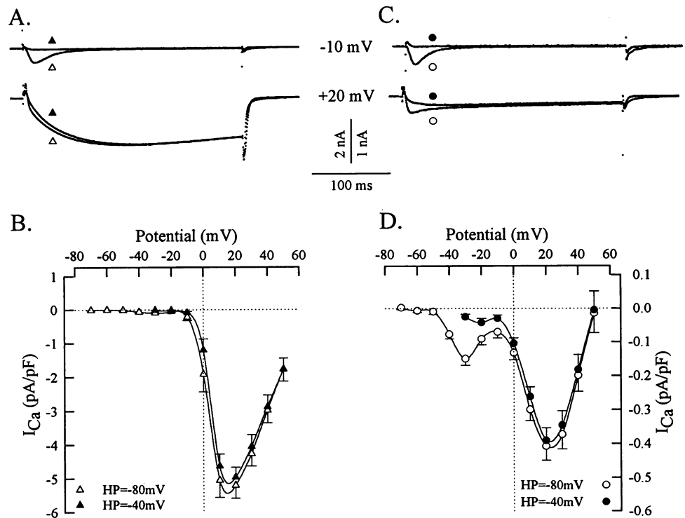
FIGURE 2 \text{Ca}^{2+} currents in normal (A) and mutant (C) myotubes. Voltage-clamp records during 300-ms depolarizing steps from holding potential -80 mV ( \circ , \Delta ) or -40 mV ( \bullet , \blacktriangle ) to the indicated potential. The capacitance of normal and mutant myotubes was 417 and 489 pF, respectively. Voltage dependence of the average \text{Ca}^{2+} current density measured at the end of the pulse from a holding potential of -80 mV ( \circ , \Delta ) or -40 mV ( \bullet , \blacktriangle ) in normal (B; n = 14 ) and mutant (D; n = 12 ) myotubes.
