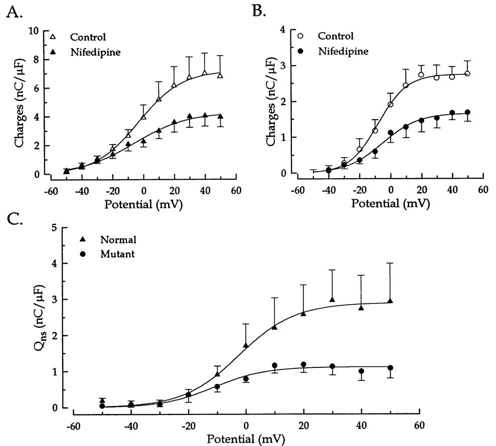
FIGURE 7 Q - V curves of normal (A; n = 6 ) and mutant (B; n = 5 ) myotubes during control ( \circ, \triangle ) and 5 min after addition of nifedipine ( \bullet, \blacktriangle ). (C) Q_{ns} - V curves of normal ( \blacktriangle , n = 6 ) and mutant ( \bullet , n = 5 ) myotubes. For each cell, Q_{ns} was calculated by subtracting the value of Q obtained after addition of nifedipine from the value of Q obtained in control at each voltage. Curves correspond to a Boltzmann fit of the mean with parameters Q_{max} = 2.89 and Q_{max} = 1.12 nC/ \mu F; V_{1/2} = -2.43 and V_{1/2} = -11.25 mV; k = 9.7 and k = 8.72 mV for normal and mutant, respectively.
