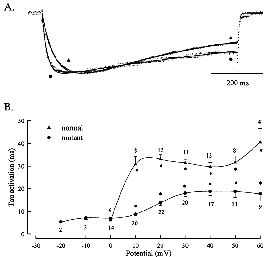
FIGURE 5 (A) Scaled traces of Ca^{2+} current from a normal (▲) and a mutant (●) myotube in response to a 750-ms depolarizing pulse from a holding potential of -40 mV to +10 mV. The solid curves correspond to a fit using the biexponential equation for I(t) described in Materials and Methods with K = -1.29 pA, \tau_1 = 54.7 ms, \tau_2 = 750 ms for normal and K = -1.07 pA, \tau_1 = 19.9 ms, \tau_2 = 1416 ms for mutant. (B) Time constant for current activation for normal (▲) and mutant (●) myotubes. Numbers near symbols indicate the number of cells. Asterisks indicate time constants of normal and mutant cells found to be significantly different to p < 0.005 according to a paired t -test.
