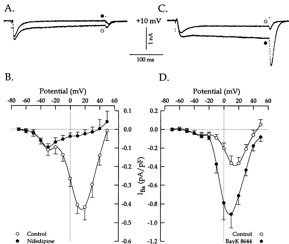
FIGURE 4 \text{Ba}^{2+} currents in response to a 300-ms depolarizing pulse from holding potential -80 mV to +10 mV in control ( \circ ) and 10 min after addition of 5 \mu\text{M} ( \bullet ) nifedipine (A) or 5 \mu\text{M} Bay K 8644 (C). The capacitance of the myotubes was 614 and 590 pF in A and C, respectively. Voltage dependence of the average \text{Ba}^{2+} current density measured at the end of the pulse in control and 10 min after addition of nifedipine (B; n = 9 ) or Bay K 8644 (D; n = 7 ).
