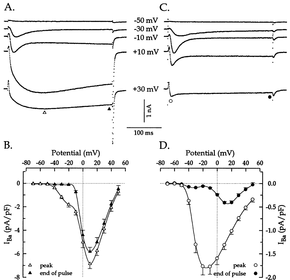
FIGURE 1 \text{Ba}^{2+} currents recorded in normal (A) and mutant (C) myotubes. Voltage-clamp records during 300-ms depolarizing steps from holding potential -80 mV to the indicated potential. The capacitance of normal and mutant myotubes was 336 and 432 pF, respectively. Voltage dependence of the average \text{Ba}^{2+} current density measured at the end of the pulse ( \bullet , \blacktriangle ) and at the peak ( \circ , \triangle ) in normal (B; n = 18 ) and mutant (D; n = 17 ) myotubes.
