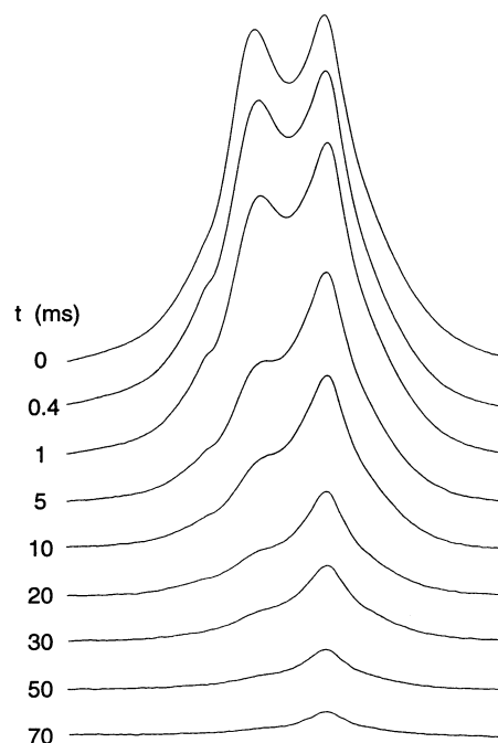
FIGURE 2 A series of 500 MHz ^1\text{H} NMR spectra from a maple shade leaf ( A. platanooides cv. "Crimson King") obtained by using the truncated CPMG pulse sequence with a fixed interval between 180^\circ refocusing pulses ( \tau = 50 \mu\text{s} ), but with variable numbers of pulses. The spectral window (total width, as displayed) is 12 ppm. Each spectrum is labeled with the total delay time, t , (i.e., the total elapsed time between the initial pulse and the FID) in ms. The peak on the right has been assigned to water in the chloroplasts, and the peak on the left to nonchloroplast water. Note that as t increases (i.e., as one goes down the series), the intensity of the nonchloroplast peak decreases more rapidly than that of the chloroplast peak.
