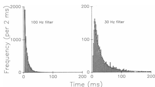
FIGURE 3 Open time distribution after exposure to PKA. Channel open times at -10 mV were computed from 192 episodes. At 100 Hz filter frequency ( left ), a total of 8,687 open events were detected. When the same calculation was carried out after a step of digital filtering at 30 Hz ( right ), the number of open events detected was reduced to 2,206. Both histograms were best fitted by a sum of two exponential distributions (Eq. 2). The best fit values of the parameters at 100 Hz were: W_1 = 20,195 , \tau_1 = 6.5 ms, W_2 = 2,929 , \tau_2 = 22.1 ms. At 30 Hz: W_2 = 4,290 , \tau_2 = 19.8 ms, W_3 = 1,114 , \tau_3 = 101 ms.
