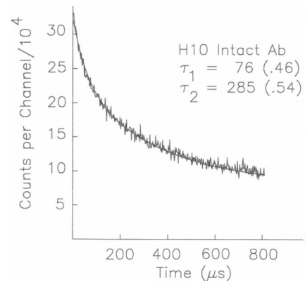
FIGURE 3 Intensity function ( \Delta I_1 + 2g\Delta I_{\perp} ) for a summed data set consisting of 20 traces plotted versus time after exciting light pulse. Each trace was obtained from single to small clumps of cells labeled with EITC-derivatized H10 Fc ε RI-specific monoclonal antibodies at 4°C. When these data were fitted to a two-exponential decay model, triplet lifetime values of 76 and 285 \mu\text{s} with fractional amplitudes of 0.42 and 0.58, respectively, were obtained.
