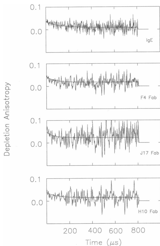
FIGURE 5 Anisotropy decays for rotation at 4°C of 2H3-RBL cell Type I Fc_{\epsilon}RI receptors binding EITC-Fab fragments of three different Fc_{\epsilon}RI -specific monoclonal antibodies (F4, J17, and H10) and EITC-IgE plotted versus time after exciting light pulse. From top to bottom the traces represent the following Fc_{\epsilon}RI ligands and numbers of summed single cell measurements: EITC-H10-Fab, 20 measurements; EITC-J17-Fab, 46 measurements; EITC-F4-Fab, 56 measurements; EITC-IgE, 76 measurements. The smooth curves are anisotropy data fitted to Eq. 6 using weighting obtained from the corresponding intensity function.
