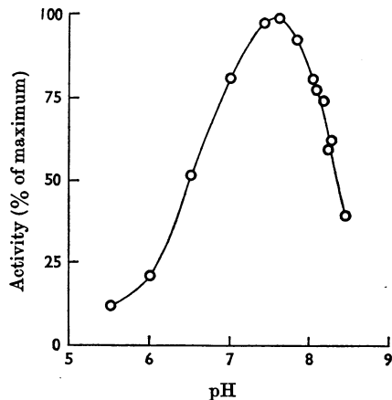
Fig. 1. pH-activity curve. Reaction mixtures contained GSH (5 mM), diethyl maleate (5 mM) and dialysed rat-liver supernatant in 0.2M-pyrophosphate buffer. Incubation was for 1 min. at 25°.
