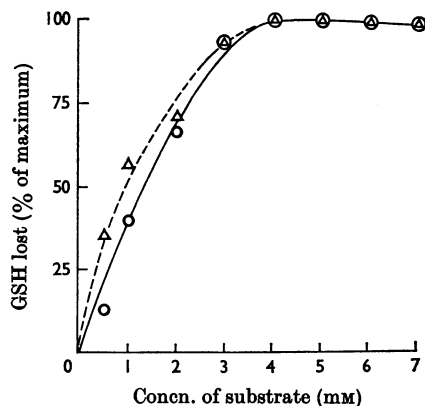
Fig. 2. Velocity-substrate concentration curves for diethyl maleate (O) in the presence of 5 mM-GSH and for GSH (Δ) in the presence of 5 mM-diethyl maleate. Incubation was for 5 min. at 25° and pH 6.5.
